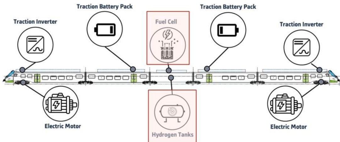
Fig. 2. Powertrain architecture of the studied hydrogen-battery hybrid train, with its main components indicated.
