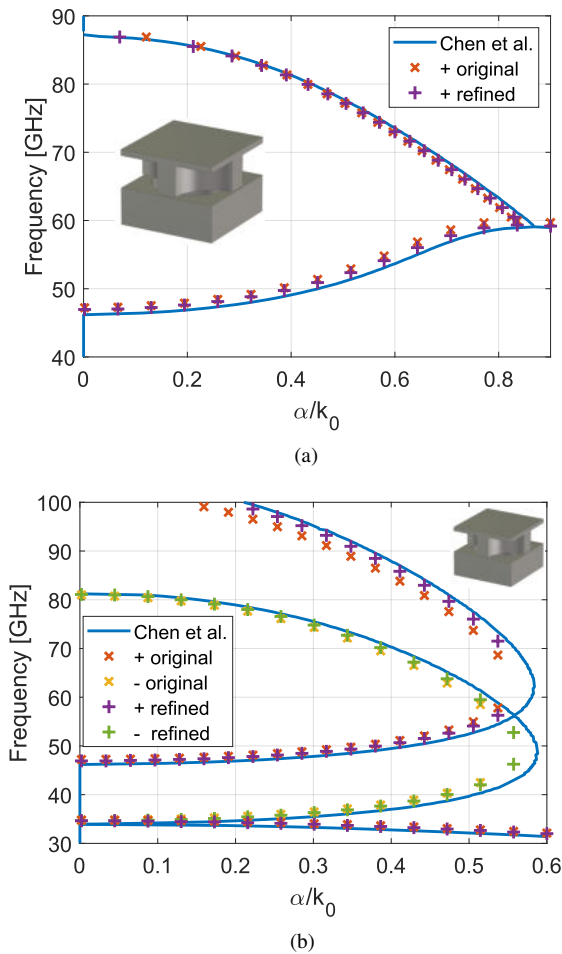
Fig. 14. (a): attenuation in the \bar{\Gamma}\bar{X} region for the glide-symmetric unit cell depicted in the inset. The solutions from 46-59 GHz are located at \Gamma and from 59-87 GHz are a complex mode with the real part presented in Fig. 13. (b): attenuation in the \bar{M}\bar{\Gamma} region for the mirror-symmetric unit cell depicted in the inset. The solutions from 49-60 GHz were found at M and from 75-100 GHz at \Gamma .
