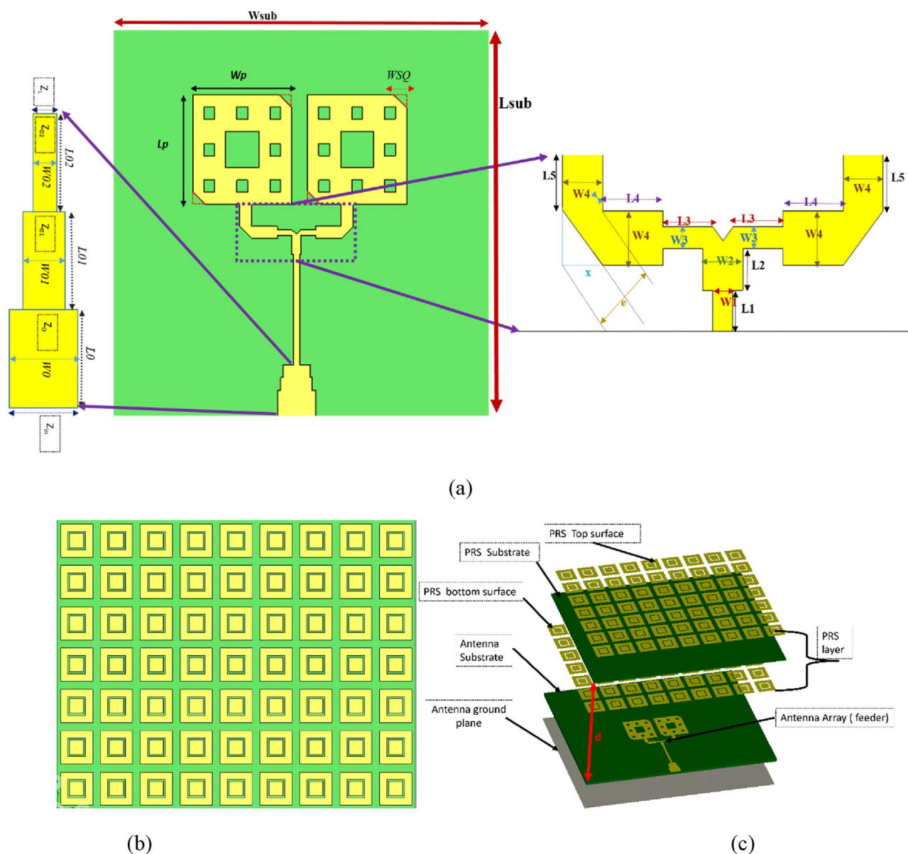
Fig. 1. Geometry of the proposed single-element antenna: (a) Front view, (b) side view, and (c) exploded view.
