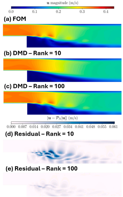
Fig. 3. Comparison between the FOM velocity magnitude and the DMD reconstruction, using 10 and 100 modes, with the associated residual field at t = 1.92 s. The figure is zoomed in on the step region.
