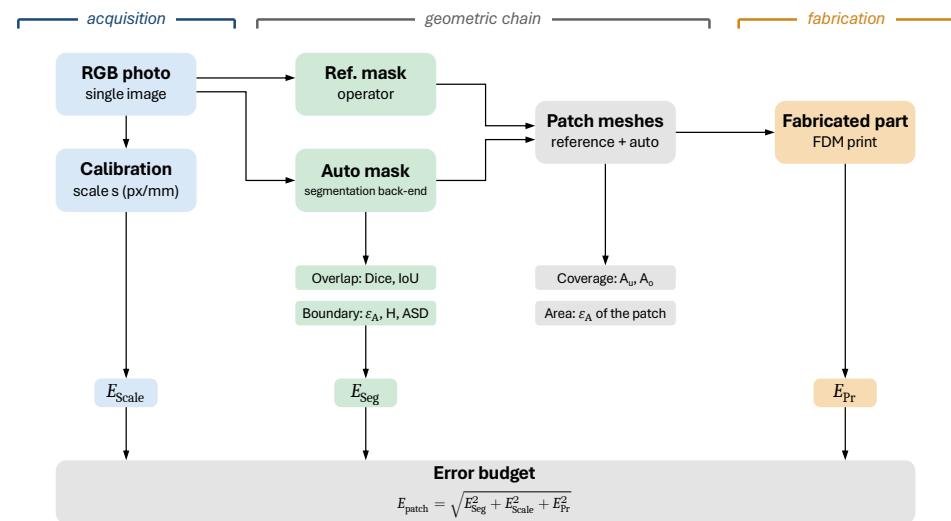
Figure 3. Data flow of the stage-wise error budget (schematic): the three terms E_{\text{Seg}} , E_{\text{Scale}} and E_{\text{Pr}} are obtained from separate experiments (Section 3.6), the first and the third by measurement and the second by simulation, not on a single image carried through the chain, and combined into the standard uncertainty of the fabricated-patch area (Equation (14)). \varepsilon_A : relative area error; H : Hausdorff distance; ASD: average symmetric surface distance; A_u , A_o : under- and over-coverage; FDM: fused deposition modelling. Box colours group the elements by stage: blue, acquisition; green, segmentation; grey, patch geometry and combination of the terms; orange, fabrication.
