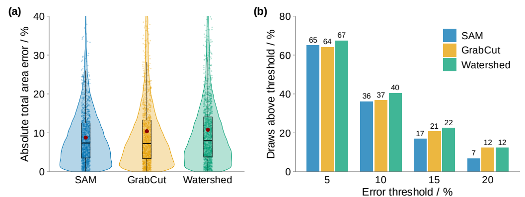
Figure 9. Monte Carlo distribution of the absolute total area error |\varepsilon_{\text{patch}}| (all valid cases; 20,000 draws per back-end): (a) distribution per back-end (violin and box computed on all draws; box: median and interquartile range; red dot: mean; dots: 1200 of the draws; 1.7% of the draws lie above the displayed 40%); (b) percentage of draws exceeding thresholds of 5%, 10%, 15% and 20%. Each draw combines a resampled clinical segmentation error with a simulated scale error and a printing error (Equation (12)); the figure therefore shows a propagated estimate, not measured clinical cases.
