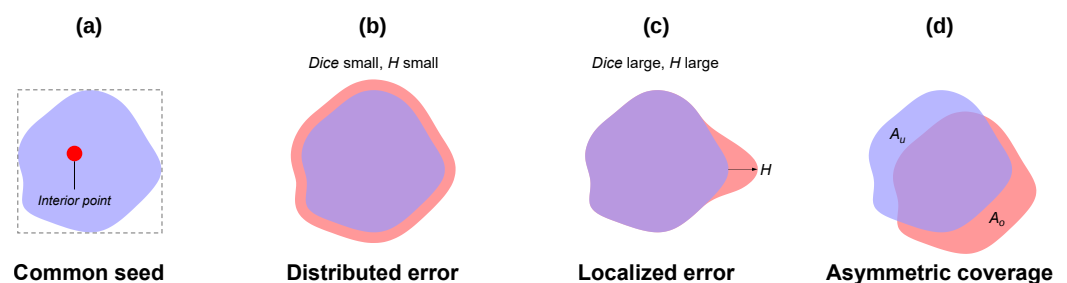
Figure 2. Concept of the fabrication-aware evaluation; in each panel the reference mask is drawn in violet and the automatic mask in red: (a) all back-ends are initialized from the operator’s reference mask (dashed box: SAM box prompt; dot: positive point at the distance-transform maximum; the classical back-ends use an eroded core of the same mask); (b,c) a disagreement distributed along the whole contour and one concentrated in a single region give different combinations of overlap (Dice) and worst-case boundary deviation (Hausdorff distance H ), so that neither metric alone describes the fabricated patch; (d) the coverage split into under-coverage A_u (reference not covered by the automatic mask, that is wound left exposed) and over-coverage A_o (automatic mask outside the reference, that is excess on healthy skin).
