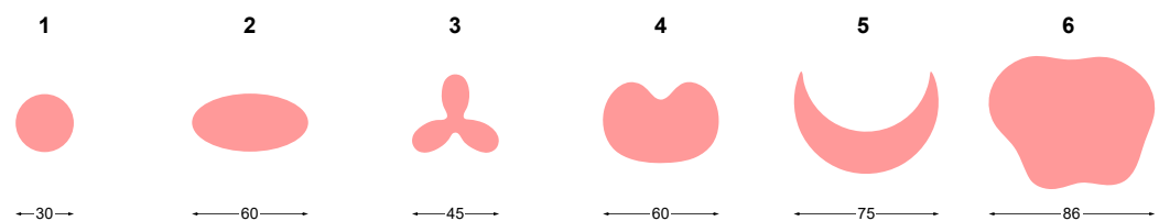
Figure 7. Nominal CAD geometries of the six planar phantom shapes of Experiments B and C, numbered 1 to 6 (disc, ellipse, trefoil, bean, crescent and freeform), with the nominal in-plane size in millimetres; each shape was printed three times in PLA by FDM (18 parts).
