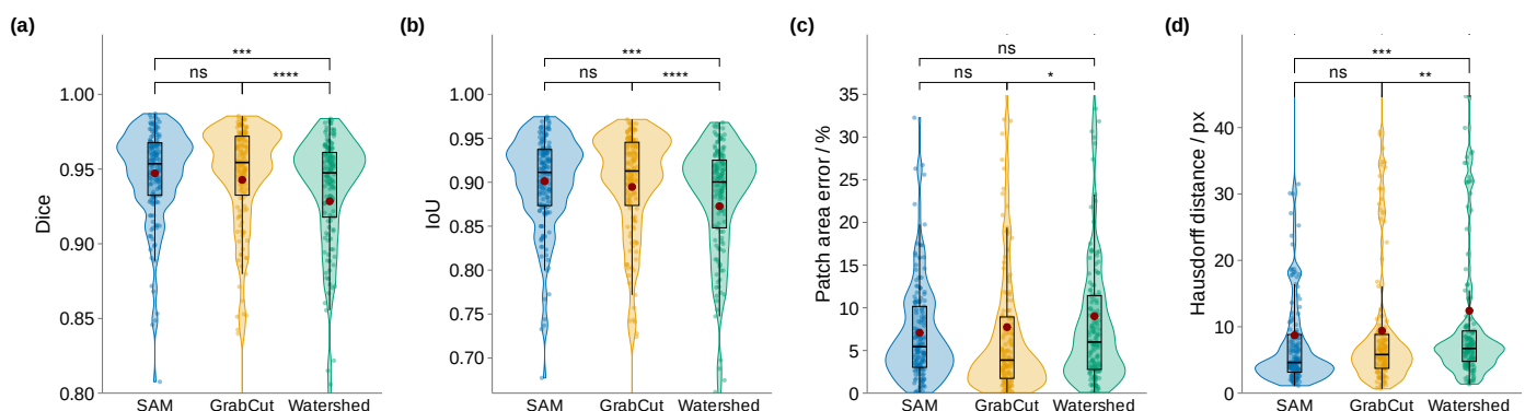
Figure 6. Per-image agreement with the reference for the three reference-seeded back-ends, all valid cases ( n = 149, 149 and 146 for SAM, GrabCut and watershed): (a) Dice coefficient; (b) IoU; (c) patch area error; (d) Hausdorff distance, in pixels because the images are uncalibrated. Violins show the distribution, boxes the median and the interquartile range, red dots the mean. Brackets give the Bonferroni-adjusted paired Wilcoxon results on the 146 images common to the three back-ends (ns: not significant; * p < 0.05 ; ** p < 0.01 ; *** p < 0.001 ; **** p < 0.0001 ). The vertical axes are truncated for readability: 8, 7, 9 and 10 of the 444 points lie outside the displayed range in panels (a–d) and are included in all the statistics.
