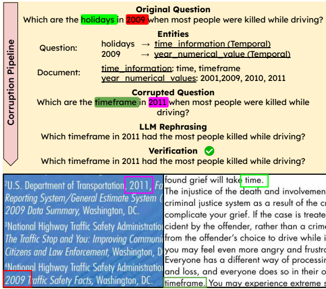
Figure 1: VRD-UQA generates unanswerable questions starting from an answerable question and the reference document. Example from DUDE (Landeghem et al. 2023)).
