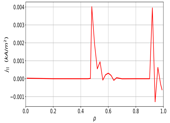
(b) harmonic n=2 is at \rho = 0.5 , n=1 at \rho = 0.95
