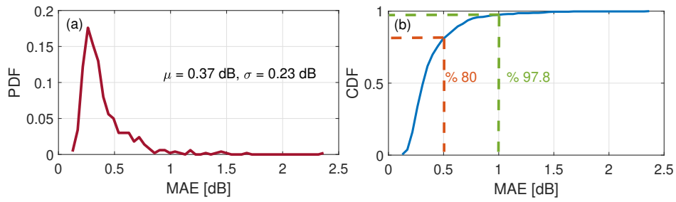
Fig. 3. The CNN model performance on test profiles. (a) PDF of the MAE, (b) CDF of the MAE.
