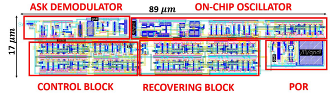
Figure 5: Final layout of the CDR system.
