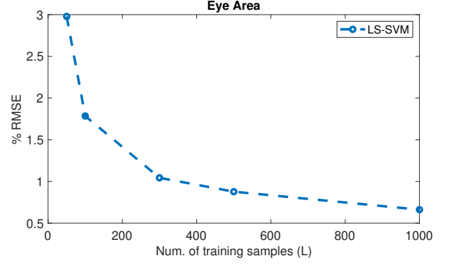
Fig. 3. Relative RMSE computed from the predictions of the surrogate models trained with an increasing number of training samples by considering 1000 test samples.
