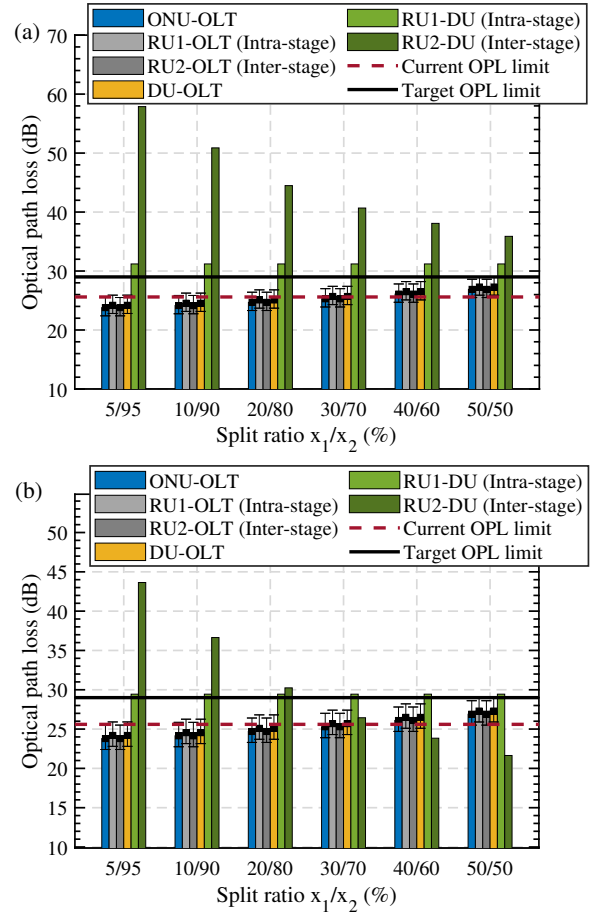
Fig. 6. Intra-PON power budget analysis for a two-stage PON splitting architecture: (a) 1:4 splitter followed by 1:16, with fiber segments of 10, 5, and 5 km; (b) 1:16 splitter followed by 1:4, with fiber segments of 15, 4, and 1 km. Intra-stage: RU in the same stage-2 branch as the DU. Inter-stage: RU in a different stage-2 branch from the DU.
