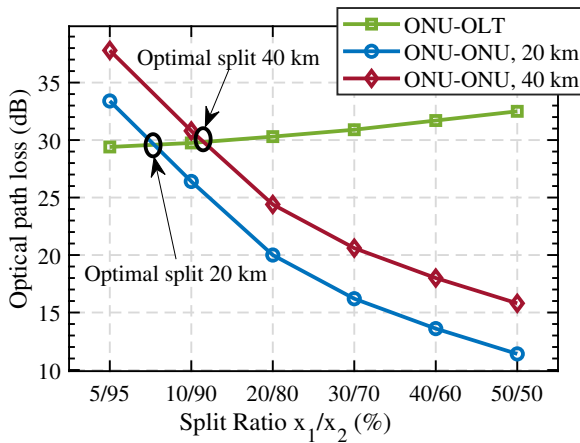
Fig. 4. Power loss as a function of taps split ratio in a one-to-one intra-PON connection with a single-stage splitter.
