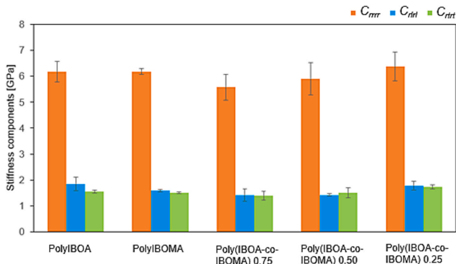
Fig. 8. Shear stiffness components C_{rrrr} , C_{rtrl} , and C_{rttr} for TW samples containing polyIBOA and/or polyIBOMA. For copolymers, the IBOA molar fraction is indicated in the x axis.
