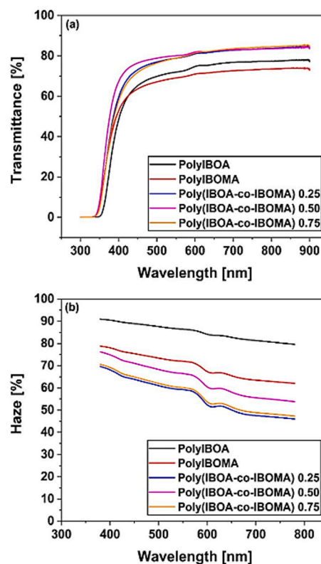
Fig. 5. Spectral optical properties of TW based on polyIBOA, polyIBOMA and their copolymers: (a) optical transmittance and (b) haze as a function of wavelength. For copolymers, the IBOA molar fraction is indicated in the legend.
