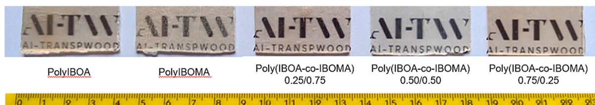
Fig. 4. Typical images of TW samples containing polyIBOA, polyIBOMA and their copolymers.
