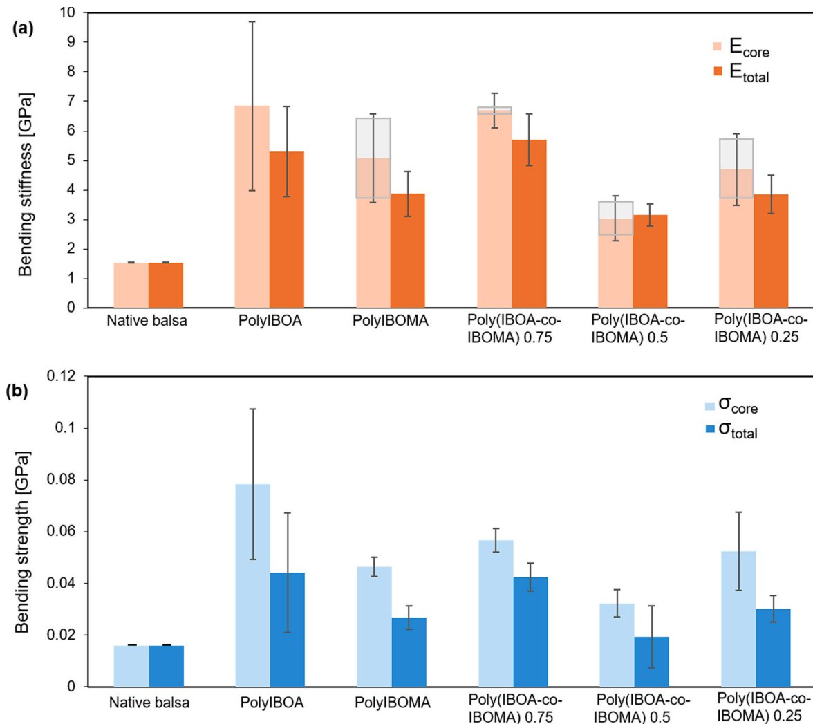
Fig. 7. (a) Bending stiffness and (b) bending strength of the total sample and the TW core, respectively, for native balsa and TW samples containing polyIBOA and/or polyIBOMA. The grey shaded area indicates the variation in the calculated E_{core} caused by varying the assumed polymer-layer stiffness. For copolymers, the IBOA molar fraction is indicated in the x-axis.
