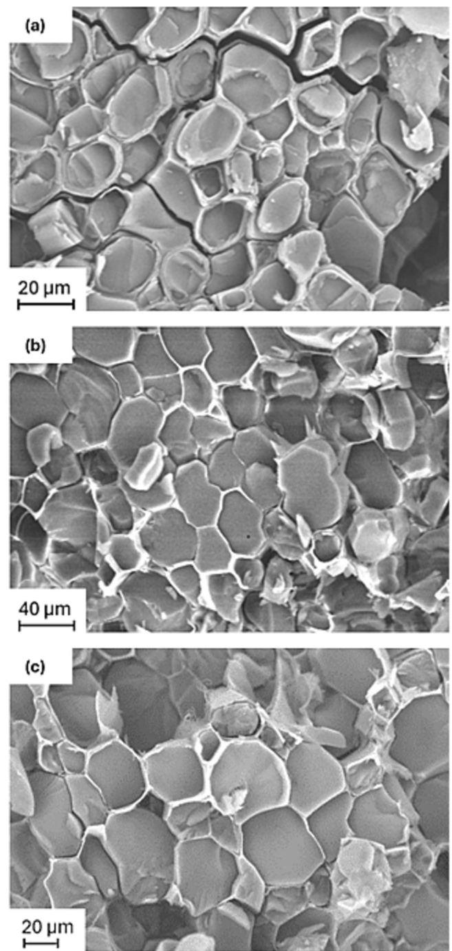
Fig. 6. Cross-sectional SEM image of TW samples embedded with (a) poly-IBOA, (b) polyIBOMA, and (c) copolymer containing an IBOA molar fraction of 0.50.
