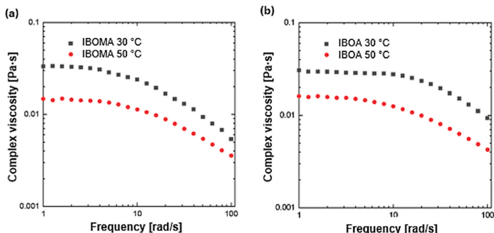
Fig. 2. Complex viscosity vs. angular frequency for IBOMA (a) and IBOA (b), at 30 and 50 °C.
