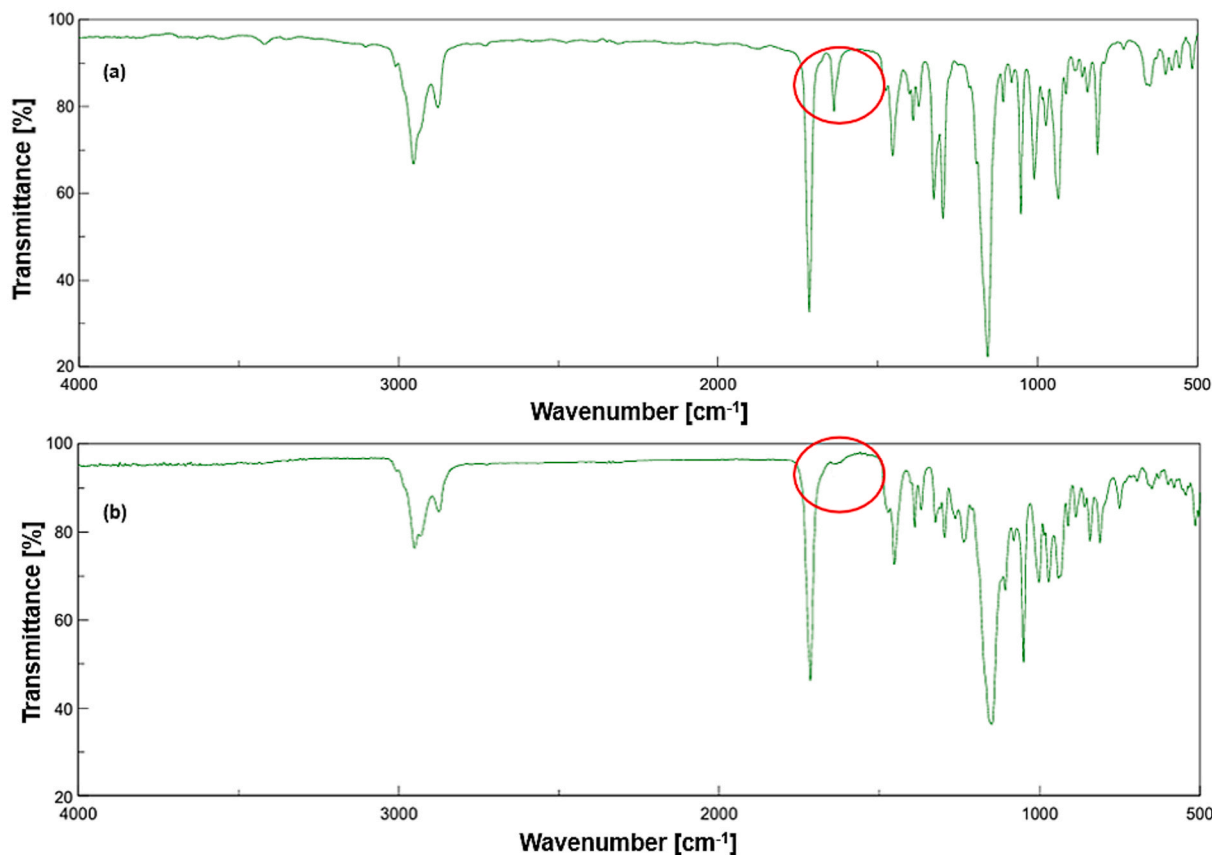
Fig. 3. FTIR spectra of IBOMA (a) and polyIBOMA (b). The graphs highlight the area corresponding to the absorption peak of the C=C bond. In the monomer spectrum the peak is clearly visible, while in the polymer spectrum it disappears.
