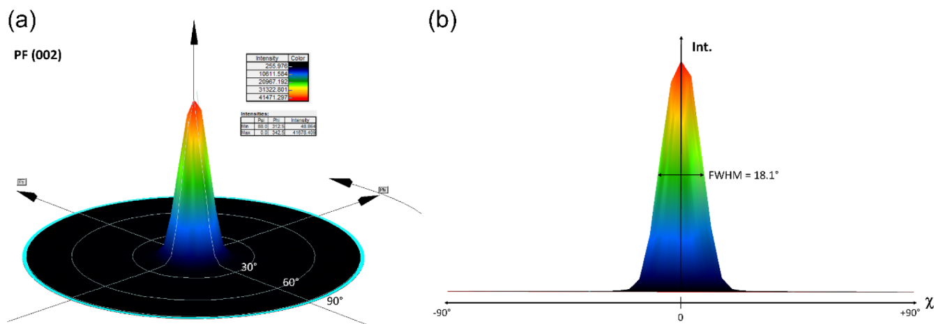
Figure 4. Pole figure analysis of a PEA 4 BiI 7 thin film based on the (002) reflection; (a) three-dimensional tilted view of the pole figure; (b) side view ( \chi -profile) showing the angular spread of the out-of-plane texture, with a full width at half maximum (FWHM) of 18.1°.
