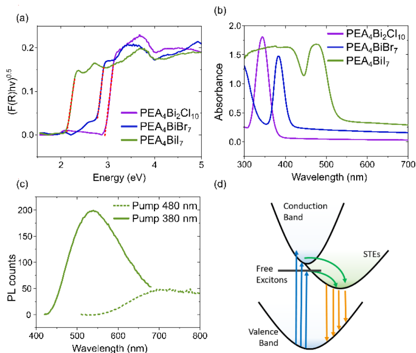
Figure 5. (a) Energy bandgaps of PEA 4 Bi 2 Cl 10 , PEA 4 BiBr 7 , and PEA 4 BiI 7 powder pellets using the reflection-mode UV-Vis measurement. The red dotted lines represent the fit to experimental data. (b) UV-Vis absorption of PEA 4 Bi 2 Cl 10 , PEA 4 BiBr 7 , and PEA 4 BiI 7 thin films using the transmission mode. (c) PL spectra of PEA 4 BiI 7 thin film excited at 380 nm (solid line) and 480 nm (dotted line). (d) Illustration of the evolution of self-trapped exciton emission of PEA 4 BiI 7 .
