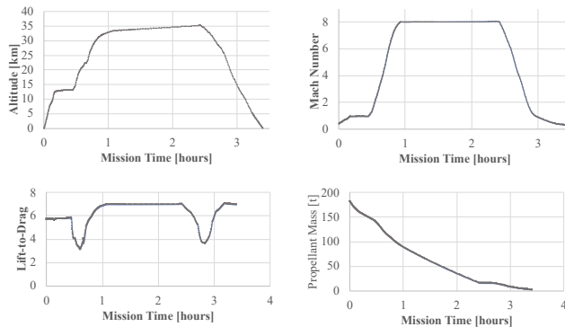
Fig. 2. STRATOFly MR3 BRU-SYD Reference Mission
