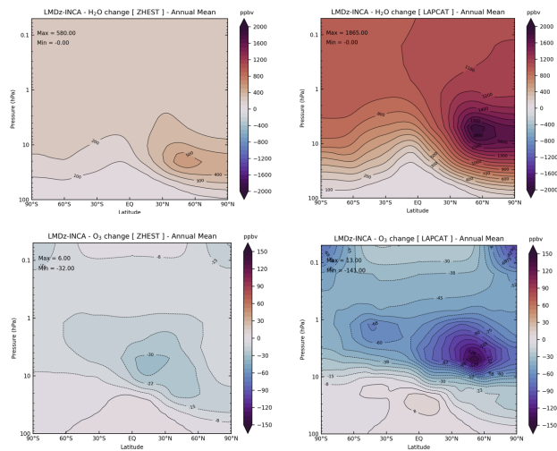
Fig. 9. Zonal mean distributions of the atmospheric water vapor and ozone mixing ratio changes (ppbv) calculated by the LMDz-INCA model and due to a fleet of hypersonic aircraft: ZEHST (left), LAPCAT (right)
