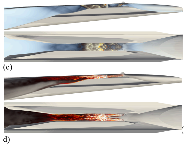
Fig. 4. Side- and top views from the combustion LES of the SSFE
