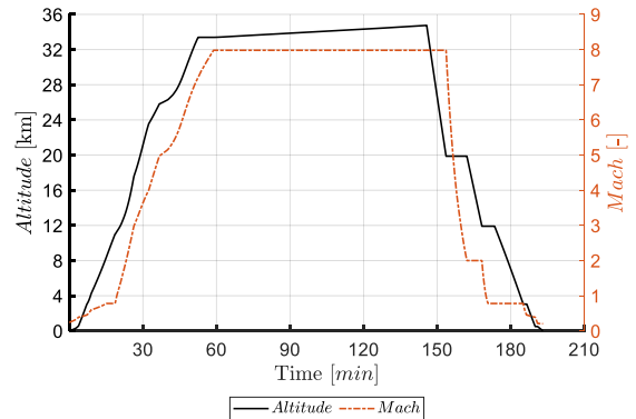
Fig. 8: Optimal altitude and Mach profile over time for MR3 with an initial cruise altitude of 109 000 ft
