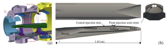
Fig. 3. The SSFE. (a) Schematic of the Small Scale Flight Experiment (SSFE) installed in the HEG test section and (b) CAD views of the computational model of the SSFE flight vehicle
