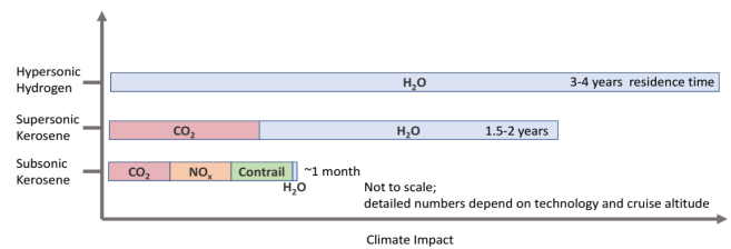
Fig. 11. Residence time of water vapor perturbation for different aircraft designs (hypersonic fueled with hydrogen, supersonic and subsonic fueled with kerosene). This representation is not to scale. Values of hypersonic vehicles are based on ZEHST and LAPCAT emissions [33]
