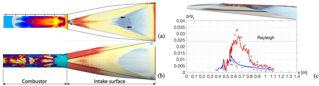
Fig. 5. Measured (a) and computed (b) wall heat flux on the lower combustor wall and on the intake.
