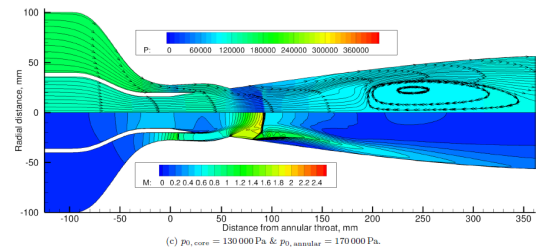
Fig. 7. CFD solution and contours of the laboratory scale nozzle for acoustic tests.
