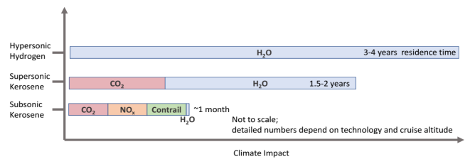
Fig. 11. Residence time of water vapor perturbation for different aircraft designs (hypersonic fueled with hydrogen, supersonic and subsonic fueled with kerosene). This representation is not to scale. Values of hypersonic vehicles are based on ZEHST and LAPCAT emissions [33]
