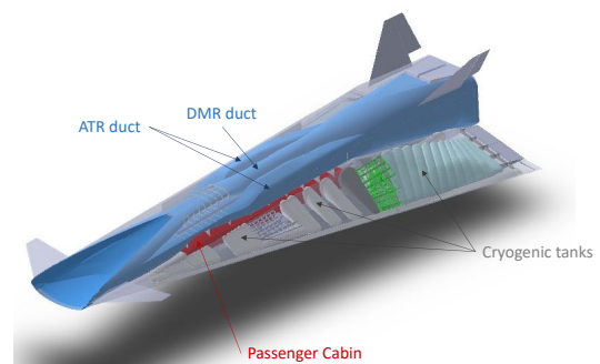
Fig. 1. STRATOFLY MR3 vehicle layout and subsystems integration
