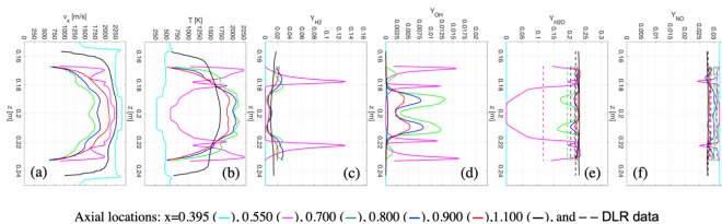
Fig. 6. Cross sectional profiles of the time-averaged quantities
