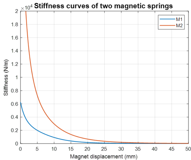
Figure 6: Stiffness curves of the two magnetic springs.
