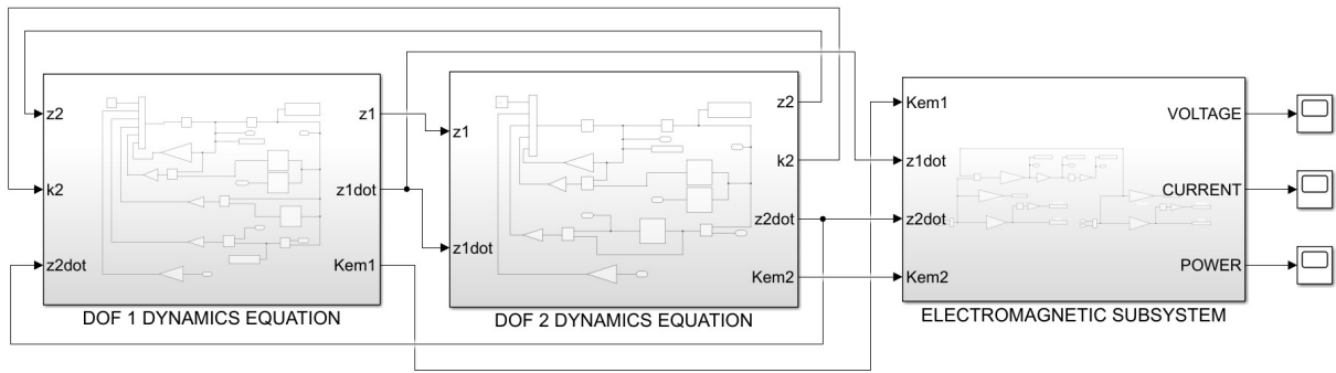
Figure 4: Simulink model.
