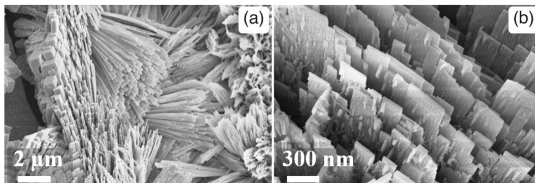
Fig. 6. FESEM micrographs of flat and non-homogeneous groups of malachite ribbons at different magnifications.
