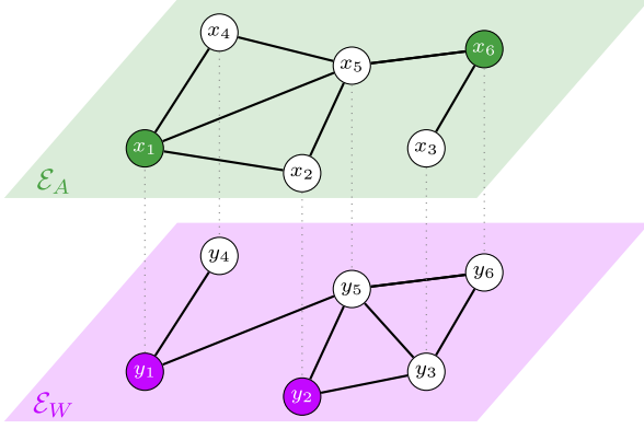
Fig. 2. Example of a setting that satisfies Assumption 2. The top layer represents individuals' action (white for -1, green for +1), the bottom layer represents individuals' opinion (shades from white for -1 to violet for +1). Control sets are \mathcal{C}^X = \{1, 6\} and \mathcal{C}^Y = \{1, 2\} .
