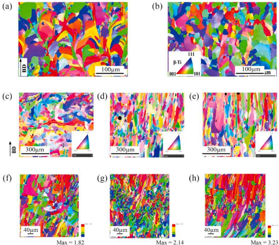
Fig. 18. EBSD maps of Zr-containing in-situ Ti alloys: (a) AS-TNZF and (b) CS-TNZF [34]; (c) Ti-29Nb-13Ta, (d) Ti-29Nb-13Ta-5Zr, and (e) Ti-29Nb-13Ta-9Zr [165]; and T3515 fabricated at (f) 250, (g) 275, and (h) 300 W [166].
