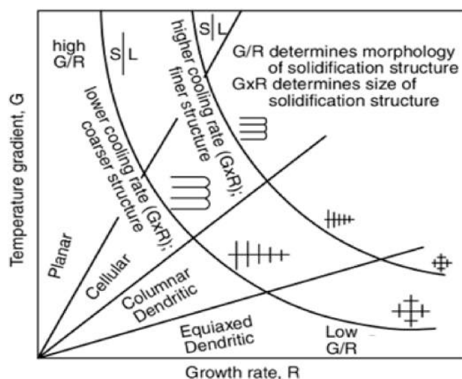
Fig. 9. Schematic G - R solidification map showing microstructure selection as a function of G and R . The G/R ratio is associated with the transition among planar, cellular, columnar dendritic, and equiaxed dendritic morphologies, while G \times R , corresponding to cooling rate, is associated with solidification structure fineness [101].
