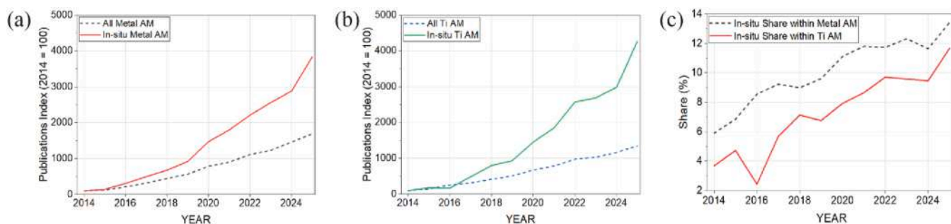
Fig. 2. Scopus-derived publication trends related to in-situ alloying in additive manufacturing: (a) indexed growth for overall metal additive manufacturing and its in-situ subset, (b) indexed growth for titanium additive manufacturing, including its in-situ alloying subset, and (c) share of in situ studies within the corresponding total literature. In panels (a) and (b), 2014 publication numbers were set to 100 for each category, so the curves show relative growth rather than absolute publication counts. Note: Scopus keyword-based queries were used; results represent indicators rather than exact counts.
