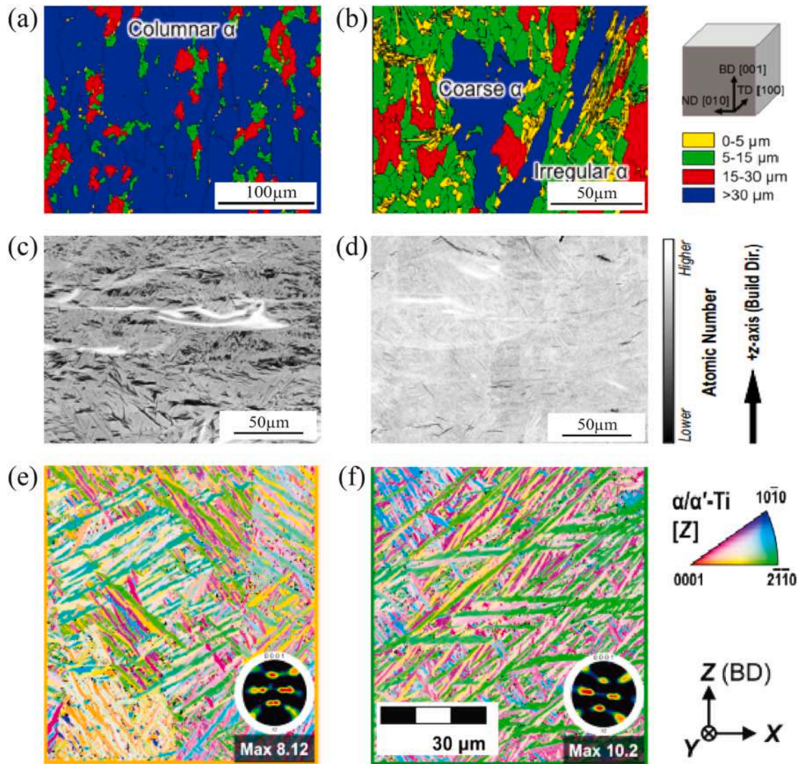
Fig. 20. Microstructural evolution of Fe-containing Ti alloys: EBSD grain-size maps of L-PBF (a) Ti and (b) Ti-0.03Fe [176]; BSE images of Ti-1Fe produced using (c) coarse and (d) fine Fe powders [177]; and EBSD IPF-Z maps of L-PBF (e) Ti-1Fe and (f) Ti-6Al-4V [178].
