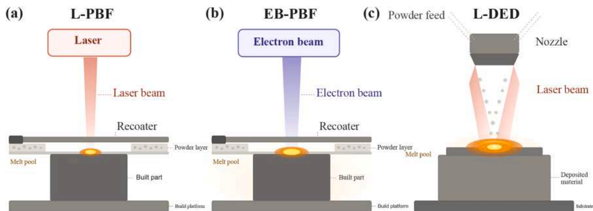
Fig. 6. Main fusion-based additive manufacturing routes used for in-situ alloying of titanium alloys: (a) L-PBF, (b) EB-PBF, and (c) L-DED.
