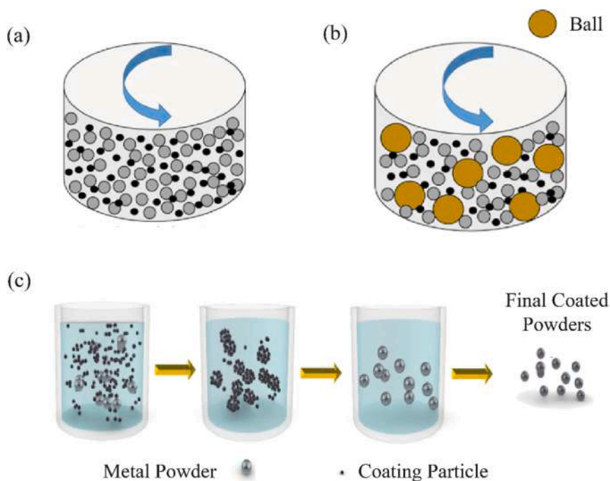
Fig. 8. Feedstock-preparation strategies for in situ alloying: (a) conventional low-energy powder mixing of a powder blend [83], (b) mechanical mixing by ball milling to promote more intimate host-guest contact, and (c) solution-based powder coating in which coating particles are deposited onto a parent metal powder to produce coated feedstock [84].
