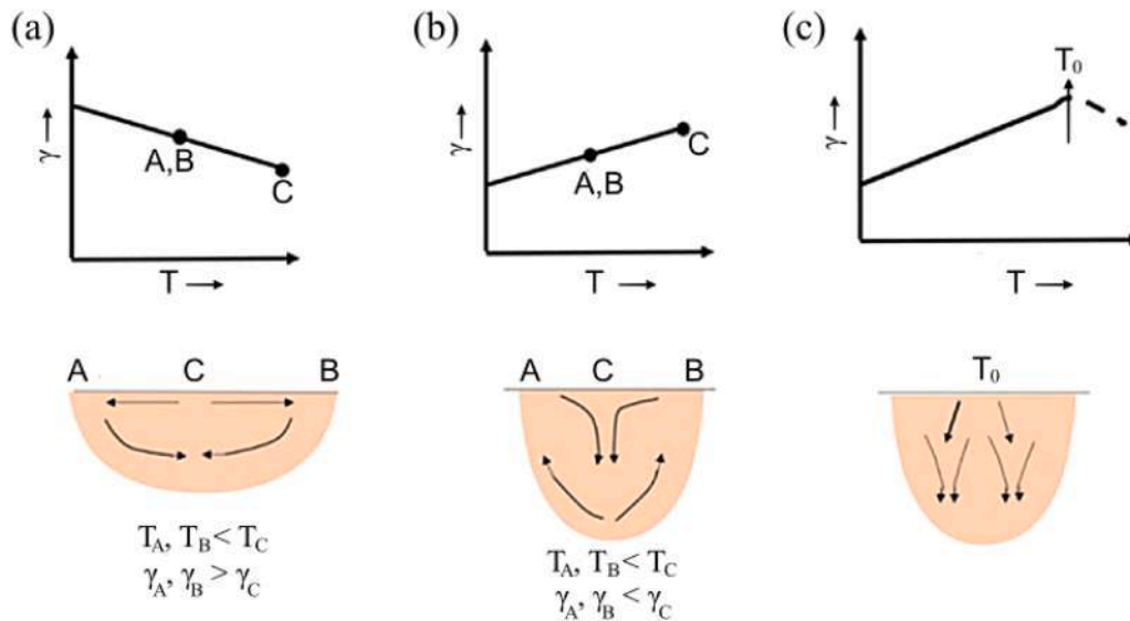
Fig. 10. Schematic Marangoni-flow patterns in a melt pool showing (a) outward surface flow for a negative surface-tension gradient, (b) inward surface flow and reversed circulation for a positive surface-tension gradient, and (c) a transitional case where the effective gradient changes sign, leading to a mixed flow response [110].
