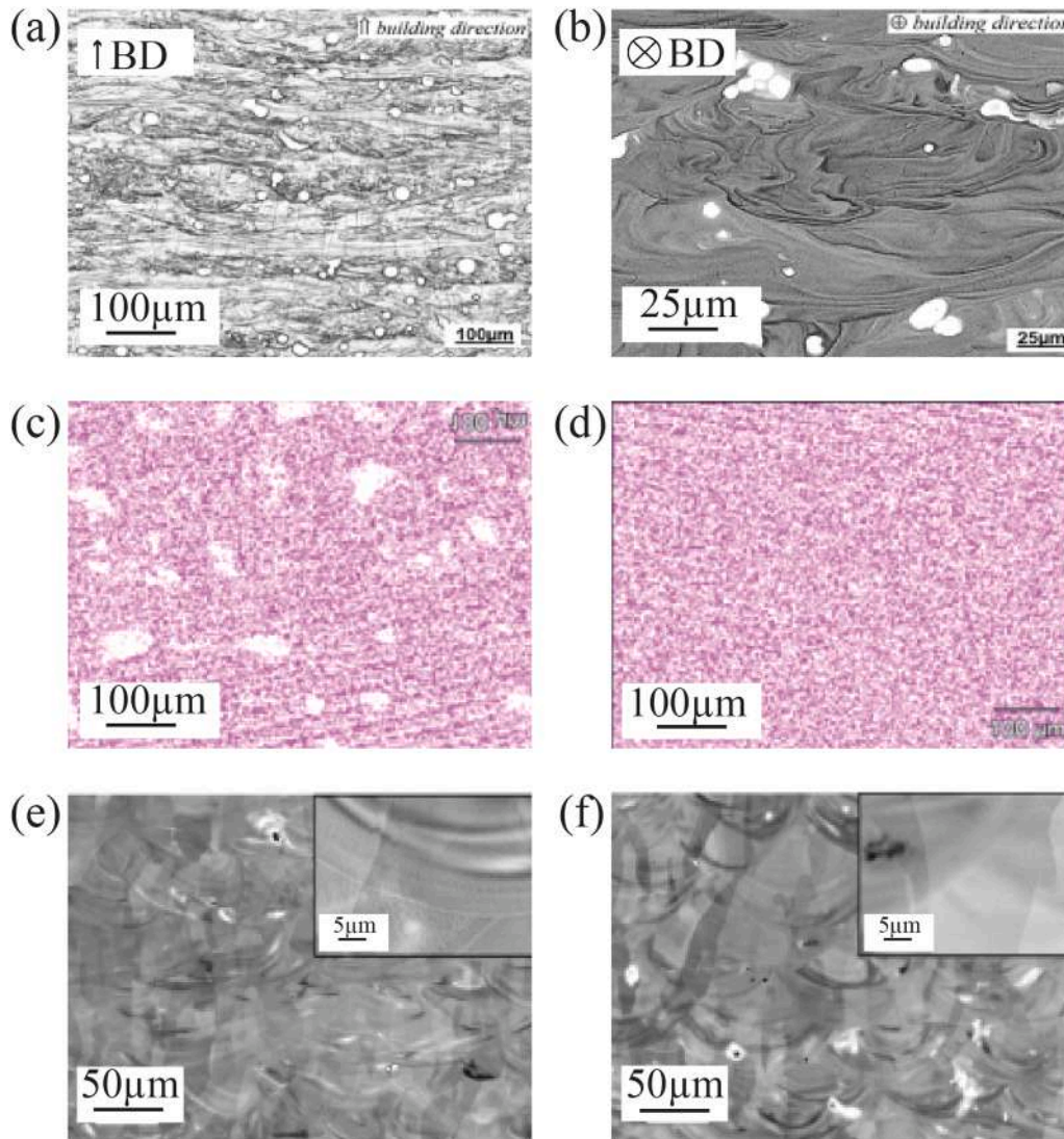
Fig. 13. Microstructural characterization of in-situ Ti-Mo alloys: (a,b) L-PBF Ti-15Mo [77], (c,d) Ti-10Mo after single and double scanning, respectively [126], and (e,f) as-built and heat-treated Ti-12Mo, respectively [130].
