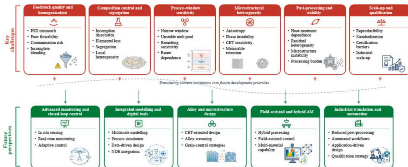
Fig. 21. Schematic overview of the main challenges and future directions for in-situ alloying of Ti alloys in fusion-based AM.
