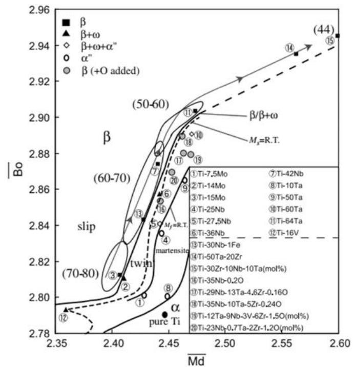
Fig. 5. Schematic Bo-Md phase stability map for \beta -type titanium alloys [25].
