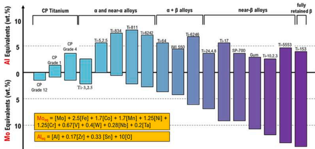
Fig. 4. Classification of titanium alloys based on Mo_{eq} and Al_{eq} values. Reproduced from [10].
