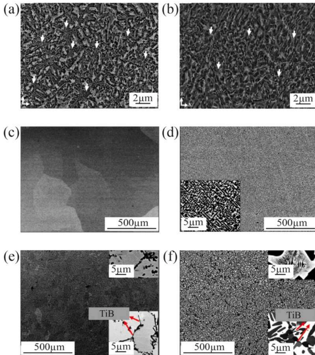
Fig. 17. Microstructures showing in-situ TiB formation in AM-processed Ti alloys: (a,b) L-PBF Ti-TiB 2 composite [155], and BSE micrographs of (c) Ti-20V, (d) Ti-12Mo, (e) Ti-20V-0.5B, and (f) Ti-12Mo-0.5B produced by LENS [158].
