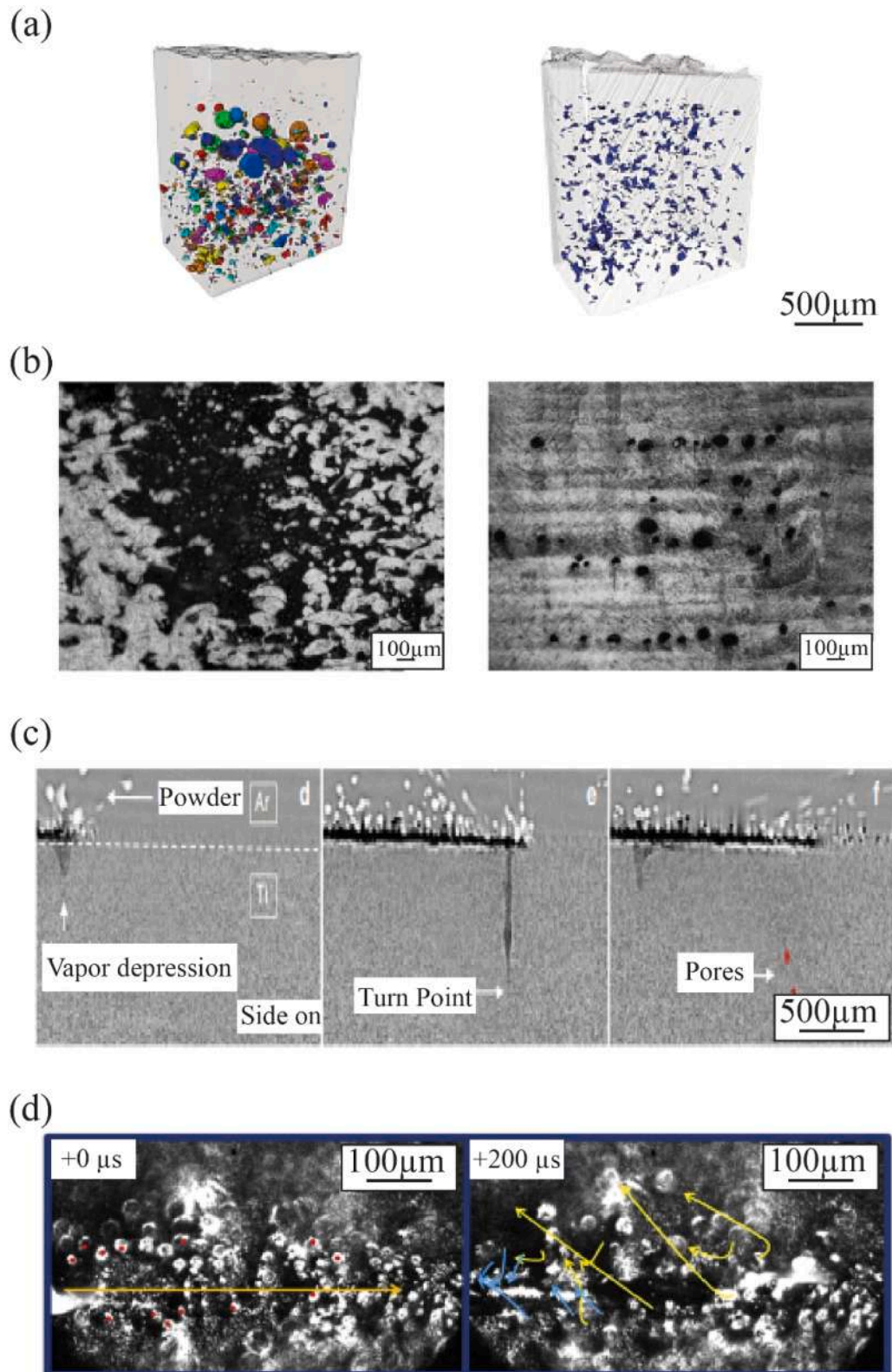
Fig. 7. Representative defects and powder bed instabilities in Ti-6Al-4V powder bed fusion. (a) Synchrotron X-ray microtomography images showing keyhole porosity, left, and lack of fusion defects, right, under different L-PBF processing conditions [67]. (b) Cross-section micrographs showing pore morphology under insufficient energy input, left, and excessive energy input, right, in L-PBF Ti-6Al-4V [68]. (c) In situ X-ray images of keyhole pore formation near a laser turn point during L-PBF of Ti-6Al-4V, shown from left to right as vapor depression formation, turn point region, and pore formation [69]. (d) High-speed imaging of powder motion around the melt track in a Ti64 powder bed, showing particle entrainment at + 0 \mu\text{s} and particle ejection and redistribution at + 200 \mu\text{s} during denudation [71].
