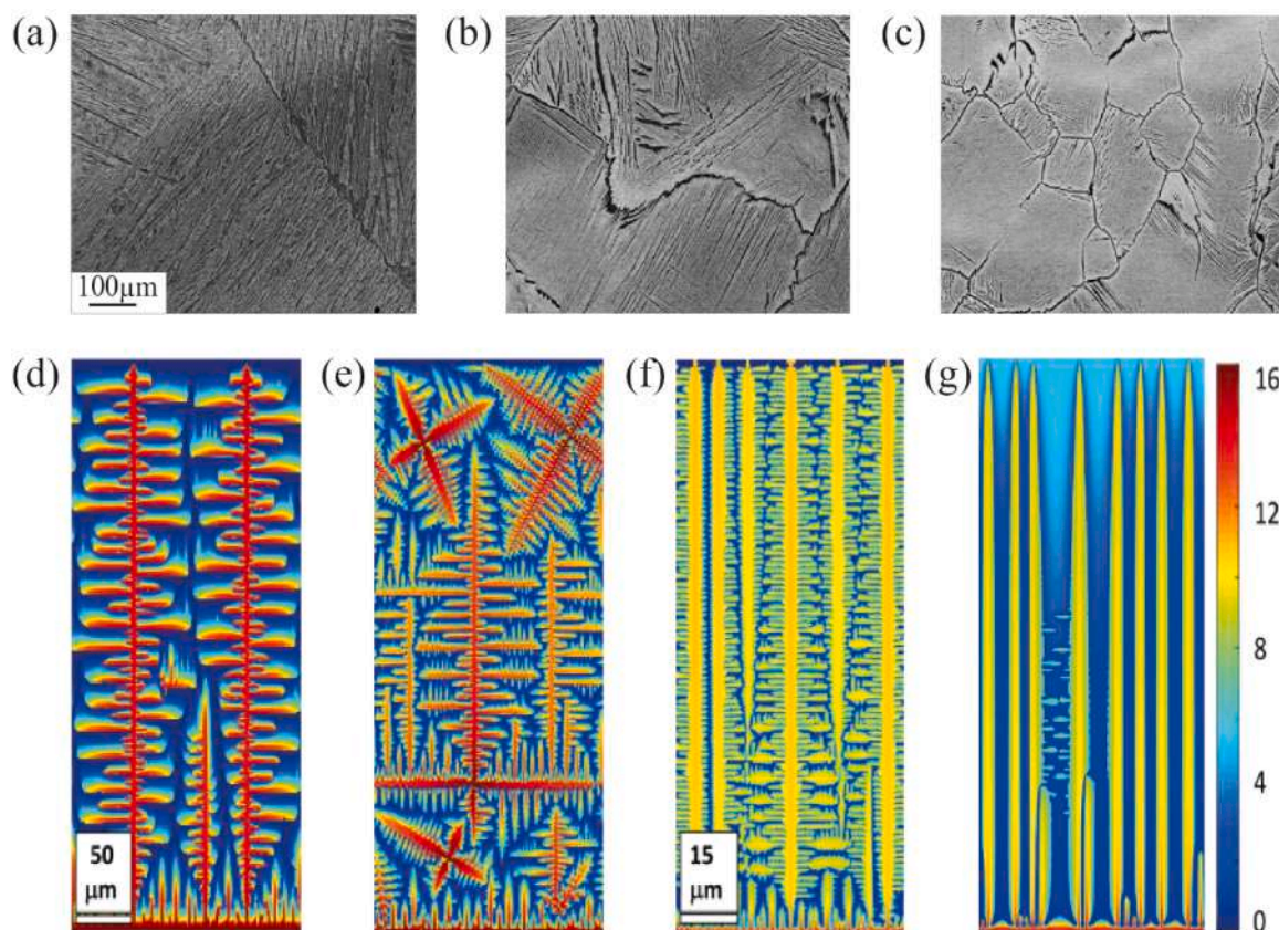
Fig. 16. Microstructural evolution of Ti-W alloys: BSE micrographs of LENS-processed (a) Ti-5W, (b) Ti-13W, and (c) Ti-25W [153]; simulated Ti-5.5 W microstructures at cooling rate/thermal gradient conditions of (d) 10 \text{ K s}^{-1} / 50,000 \text{ K m}^{-1} , (e) 50 \text{ K s}^{-1} / 50,000 \text{ K m}^{-1} , (f) 2500 \text{ K s}^{-1} / 250,000 \text{ K m}^{-1} , and (g) 4000 \text{ K s}^{-1} / 250,000 \text{ K m}^{-1} [154].
