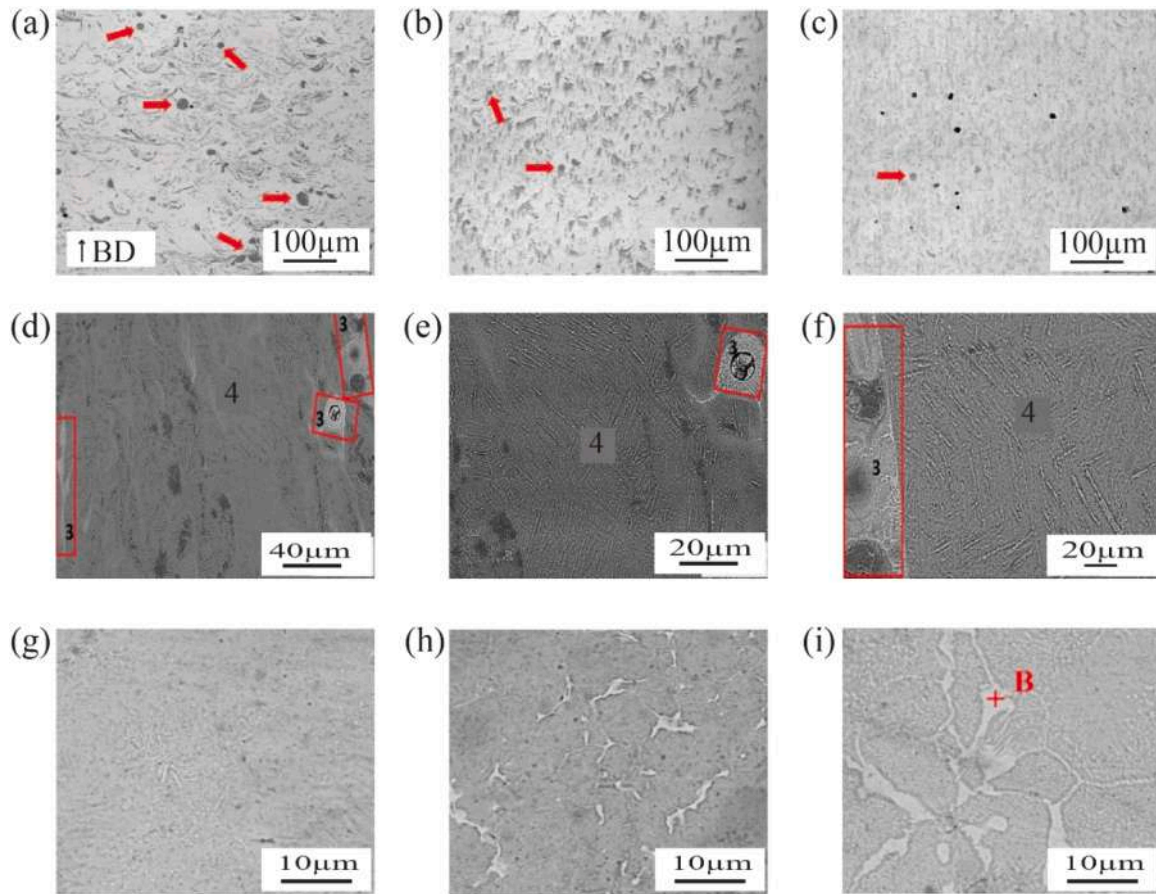
Fig. 19. Microstructures of in-situ L-PBF Ti-Cu alloys: optical micrographs at VEDs of (a) 55.39, (b) 61.68, and (c) 77.55 J mm -3 [170]; SEM micrographs of (d-f) Ti-2.5Cu [172]; and Ti-xCu with (g) 3, (h) 5, and (i) 10 wt% Cu [174].
