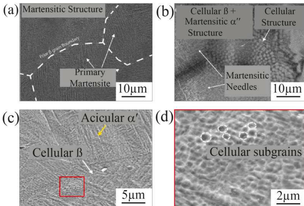
Fig. 14. Representative microstructures of in-situ L-PBF Ti-Nb alloys: (a) Ti-20Nb and (b) Ti-30Nb [134], and (c,d) Ti-25Nb [135].
