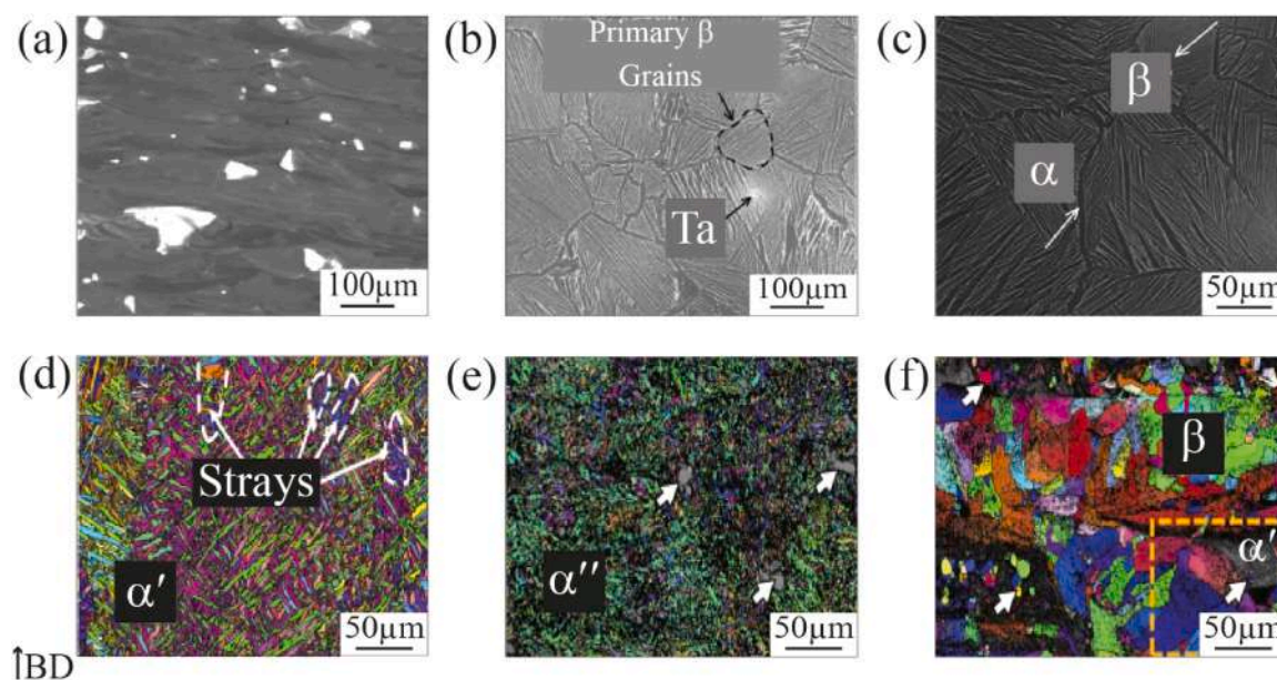
Fig. 15. Microstructural evolution of in-situ L-PBF Ti-Ta alloys: (a) as-fabricated and (b,c) heat-treated Ti-15Ta [145], and EBSD inverse pole figure (IPF)-Z maps of (d) Ti-10Ta, (e) Ti-30Ta, and (f) Ti-50Ta [147].
