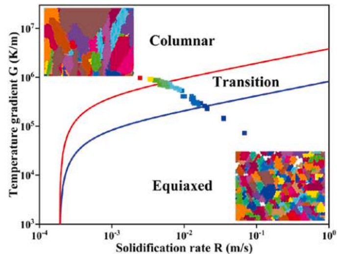
Fig. 11. G - R CET map showing columnar, transition, and equiaxed regimes as a function of G and R , with representative microstructure insets and data points crossing the transition band [114].
