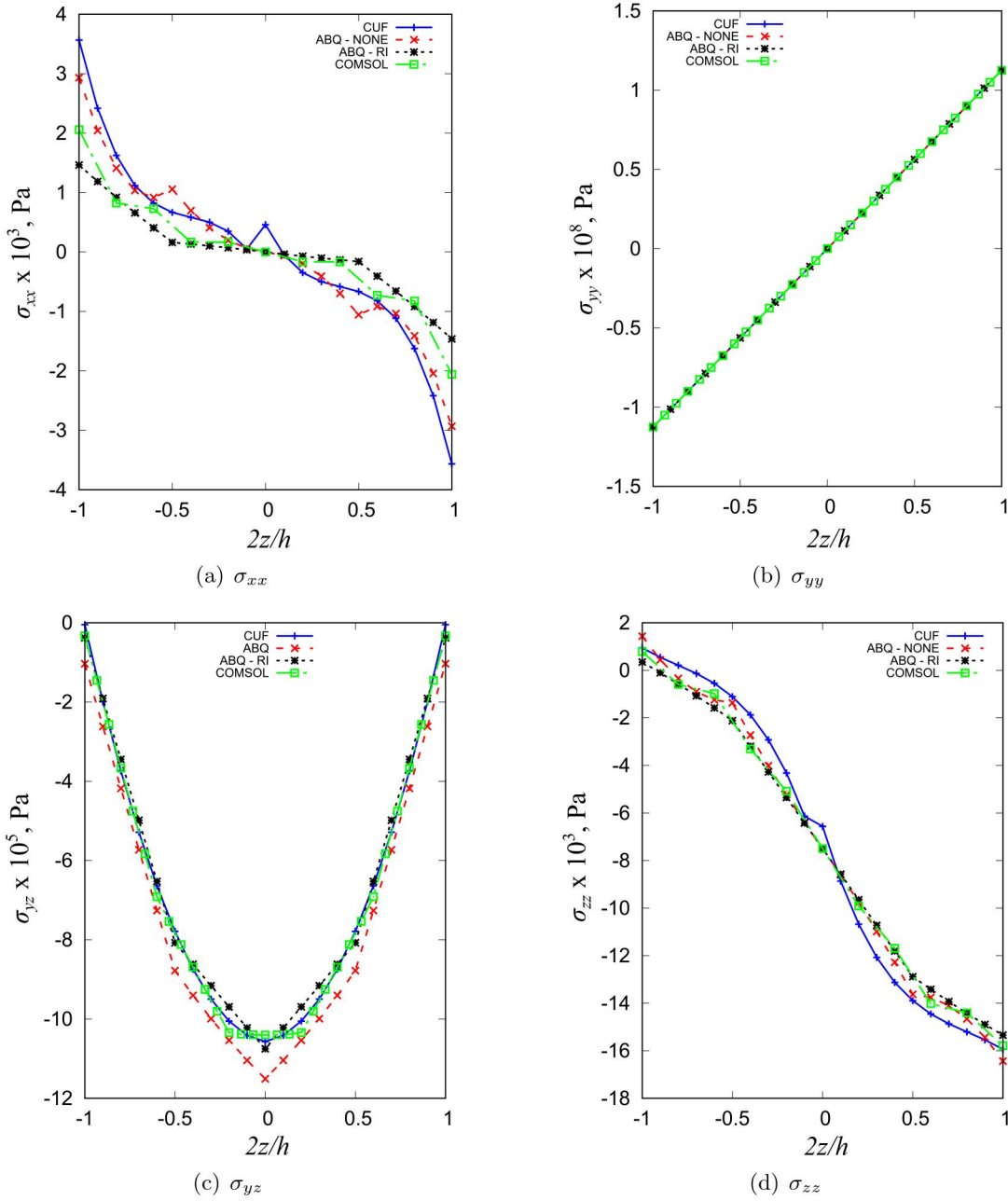
Figure 20. Comparison between CUF (AR = 10), ABAQUS (AR = 2) and COMSOL (AR = 1.2) for the through-the-thickness stress distributions for the isotropic square compact beam at the midspan.
