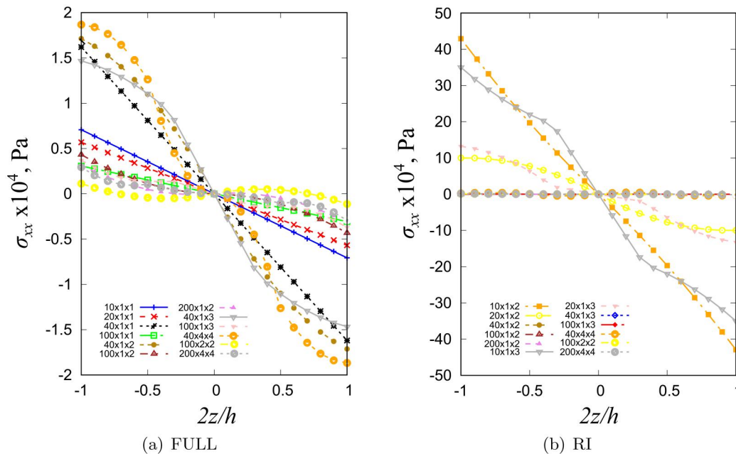
Figure 5. Through-the-thickness in-plane normal stress \sigma_{xx} distribution for the isotropic square compact beam at the midspan using ABAQUS.
