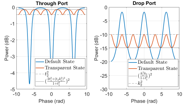
Fig. 3. Single-stage frequency response for the default and transparent state.
