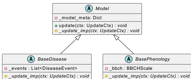
Fig. 1. UML class diagram describing the base classes of PyPlants. Green circles denote public methods, yellow diamonds denote private methods, red squares denote private attributes, and italic labels indicate abstract methods.
