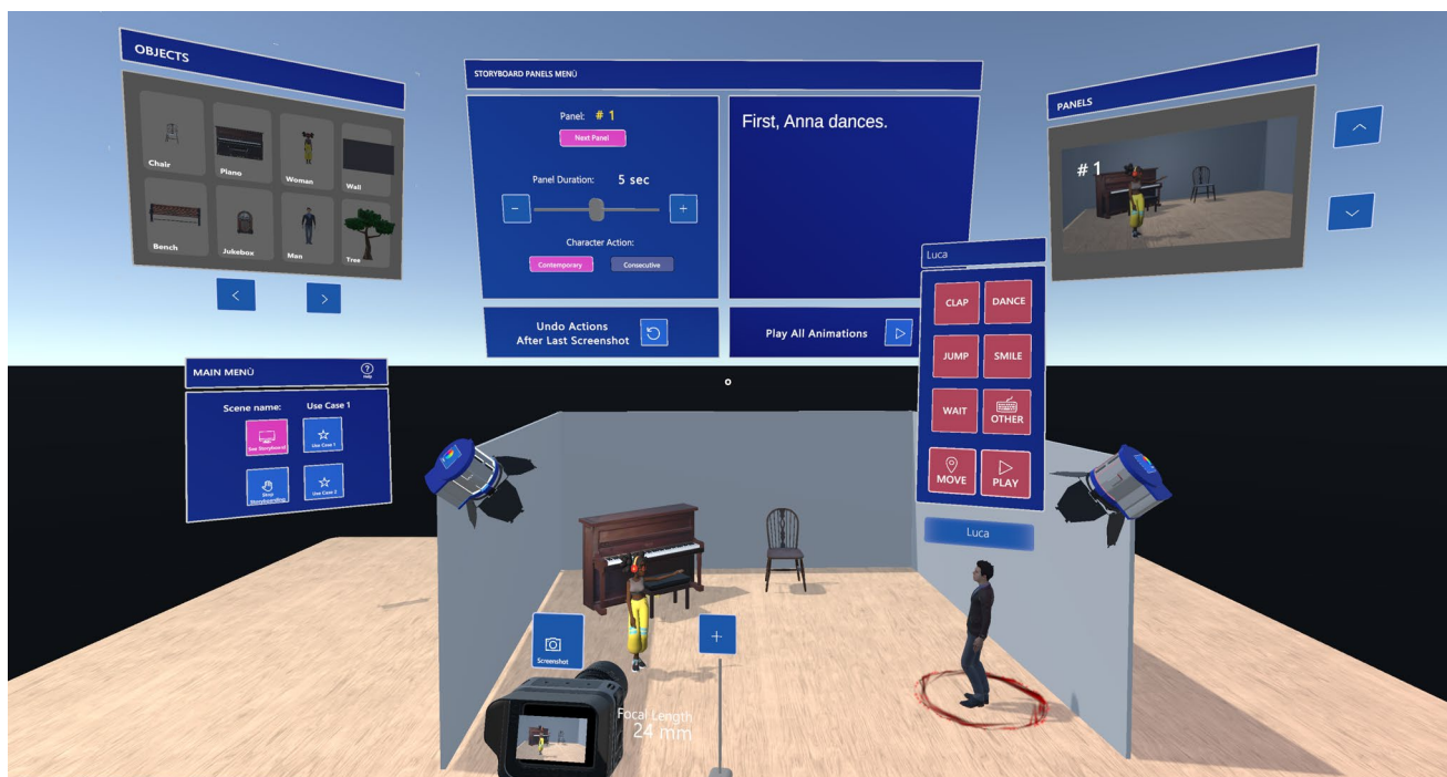
Fig. 4 The UI. All the elements of the interface are displayed: settings, characters, panels, virtual cameras, the taken screenshot, the text description, and so on
