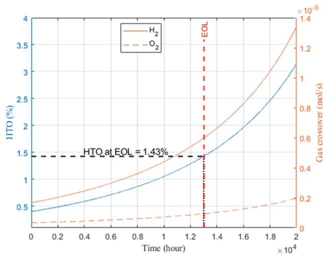
Fig. 12. Gas crossover and HTO after 20,000 h of operation.
