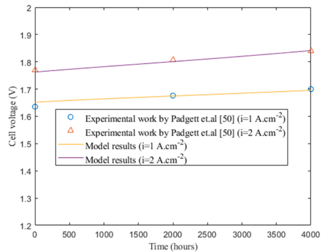
Fig. 7. Validation of the model predictions against experimental data for voltage degradation in a PEM electrolysis over an extended operating period of 4000 h (Padgett et al., 2025).
