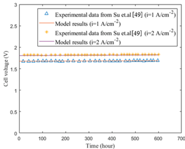
Fig. 6. Validation of model performance against experimental data for predicting voltage degradation in a PEM electrolysis cell over 600 h of operation (Su et al., 2024).
