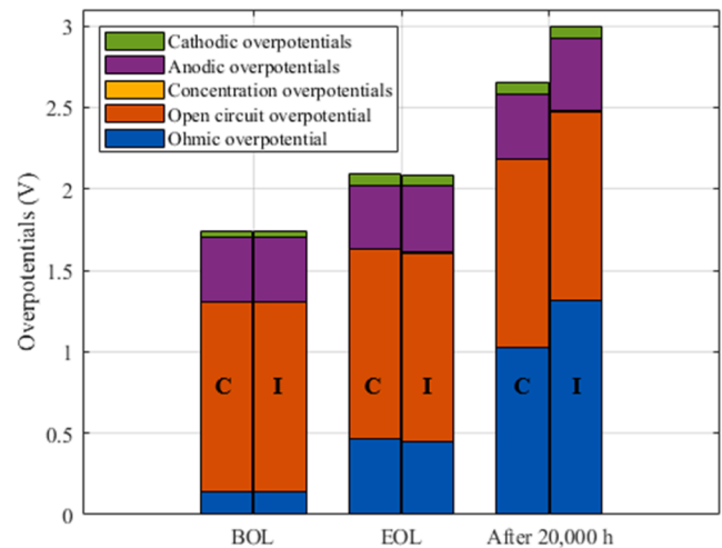
Fig. 23. Comparison of different overpotential contributions at BOL, EOL, and after 20,000 h of operation under constant-load operation (marked as C) and intermittent operation with frequent idle periods (marked as I).
