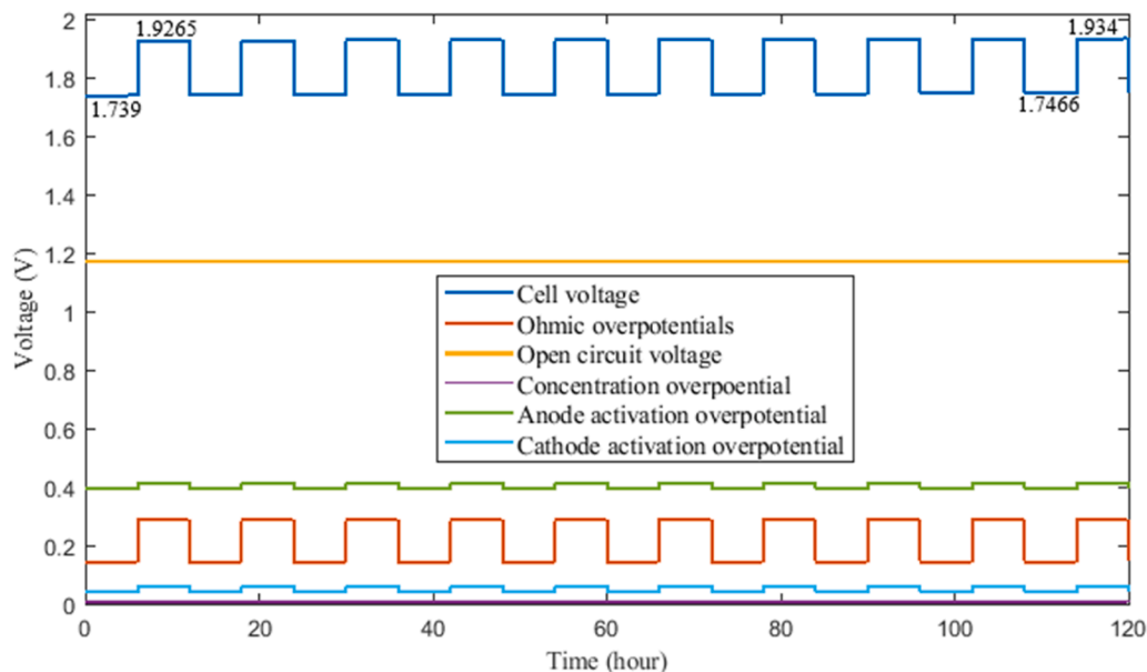
Fig. 17. The impact of LC on the cell voltage and its degradation.
