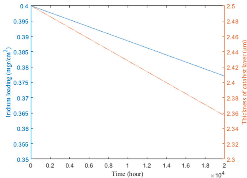
Fig. 9. Variation of the iridium loading and thickness of catalyst layer on the anode side over the time.
