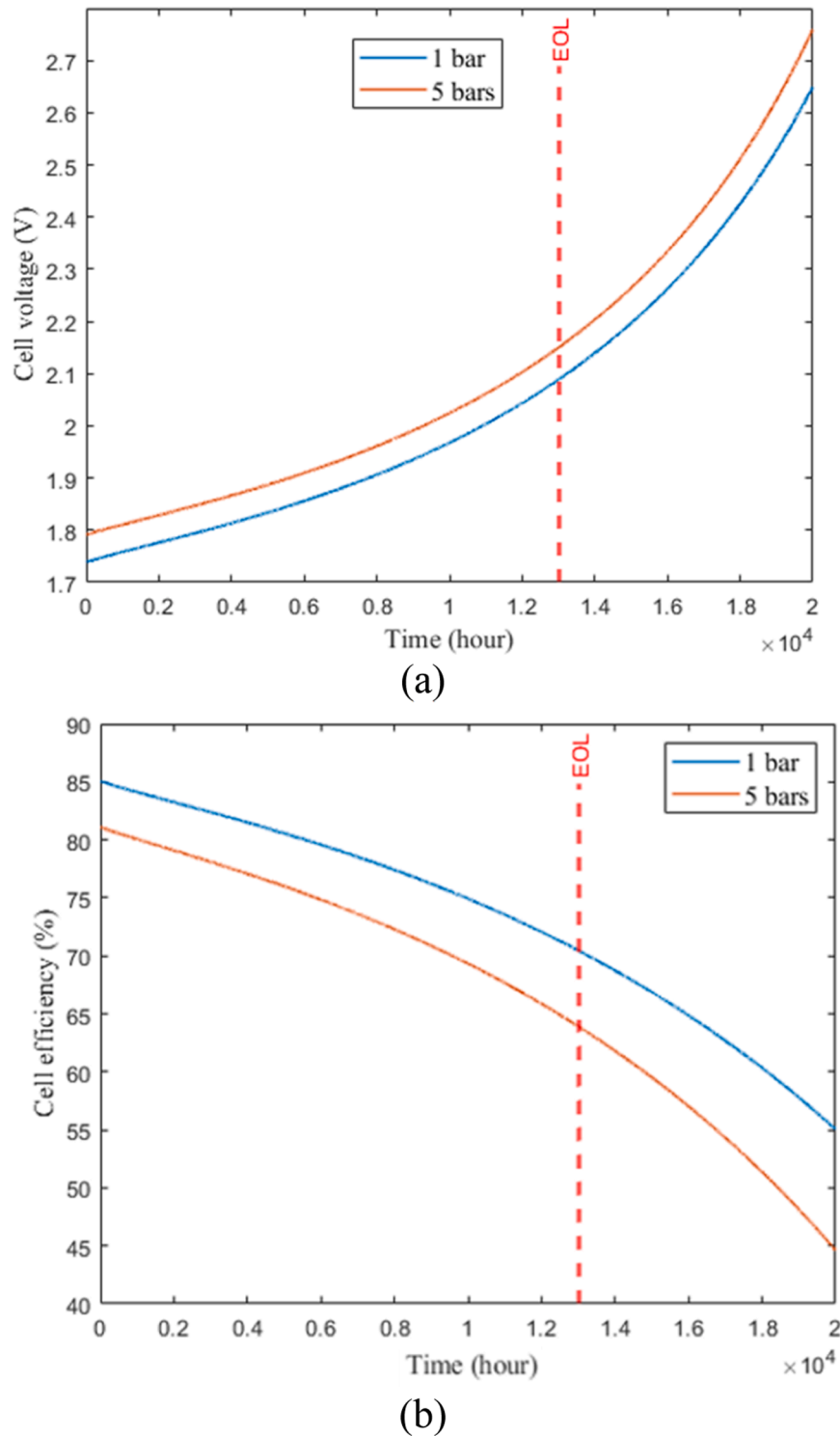
Fig. 25. The impact of operating pressure on (a) cell voltage and (b) energy efficiency of the PEM electrolysis cell over 20,000 h of operation.
