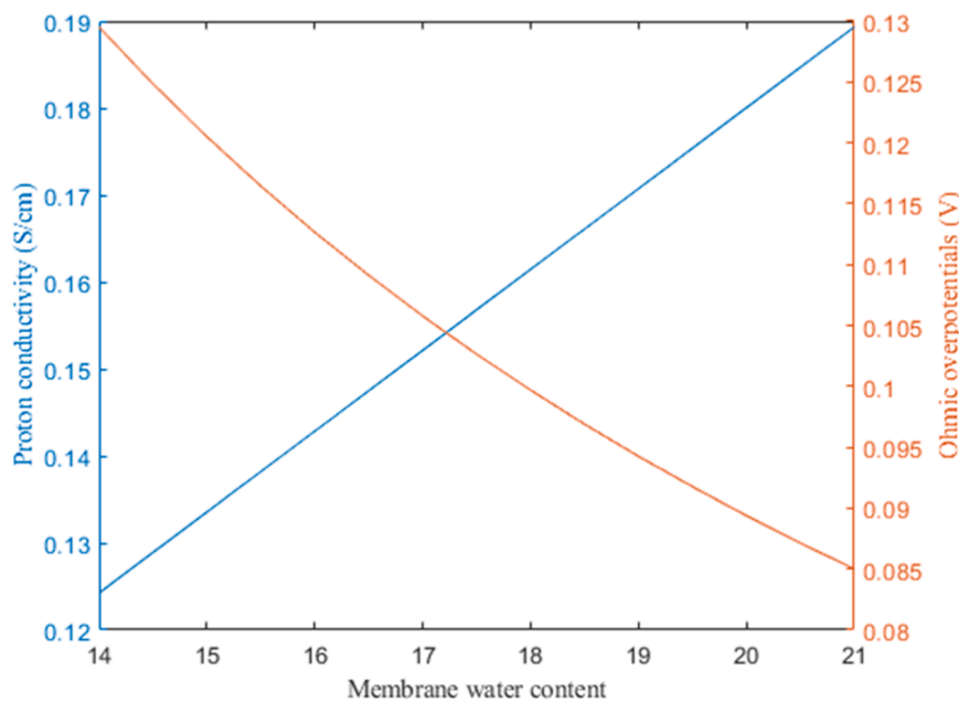
Fig. 3. Variation of proton conductivity and ohmic overpotential of membrane as a function of membrane water content.
