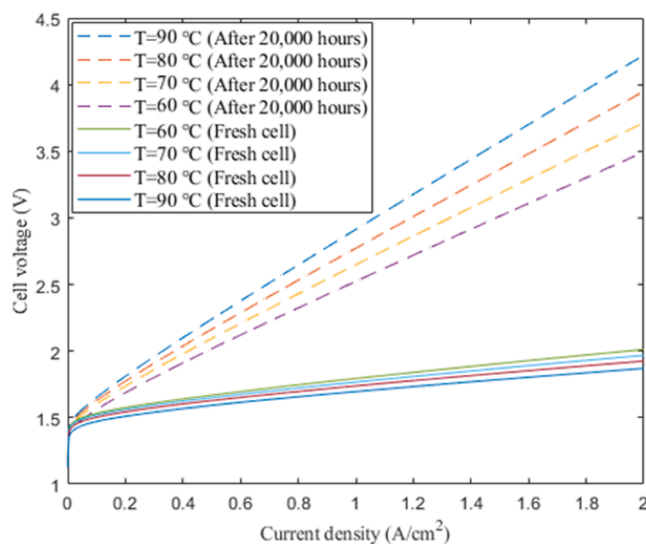
Fig. 4. Polarization of fresh cell and degraded cell after operating for 20,000 h under baseline operating conditions.
