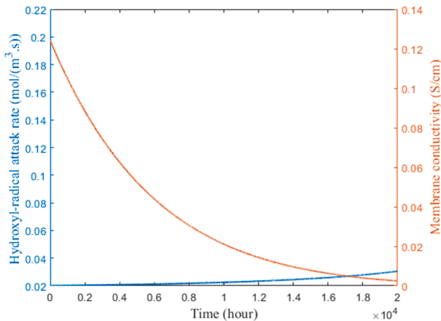
Fig. 8. Evolution of hydroxyl-radical attack rate and membrane conductivity over time.
