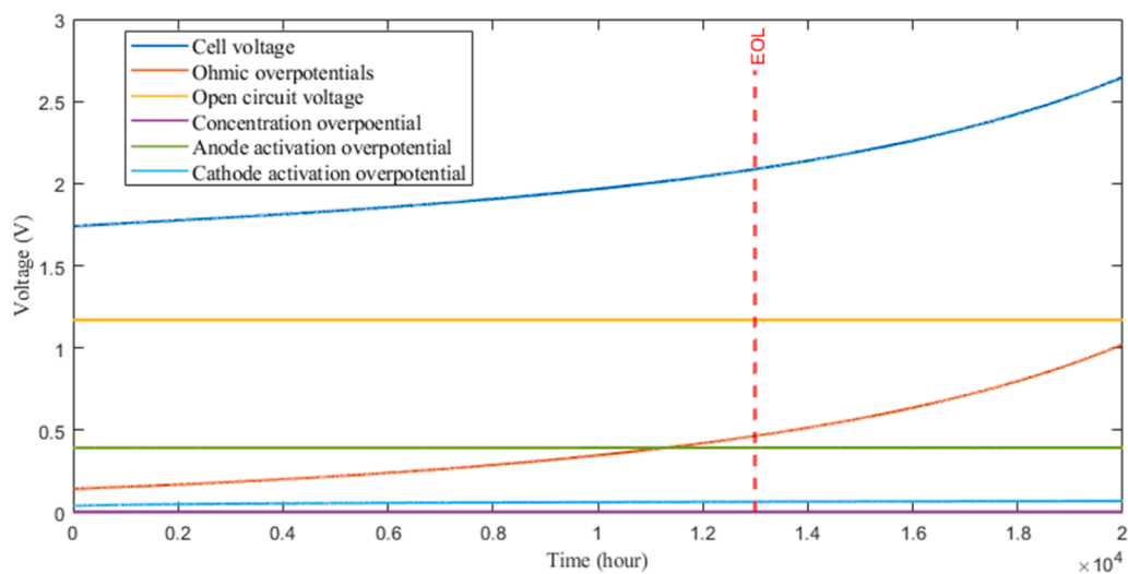
Fig. 11. Variation of cell voltage and overpotentials over 20,000 h of operation at a constant load and current density of 1 \text{ A.cm}^{-2} , and temperature of 80^\circ\text{C} .
