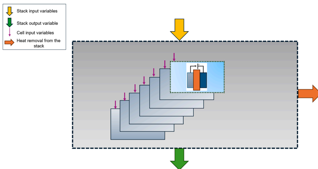
Fig. 1. Illustration of stack-level and cell-level input and output variables and associated heat removal mechanisms from the stack.
