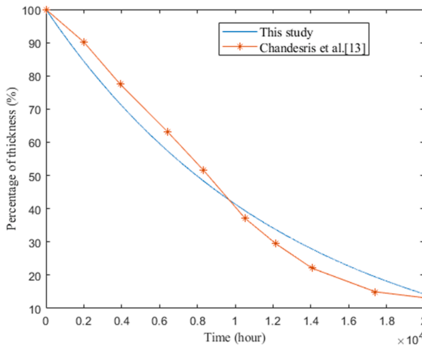
Fig. 5. Validation of model results for membrane thinning (Chandesris et al., 2015).
