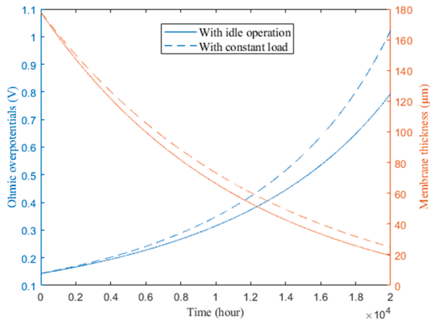
Fig. 21. Comparison of ohmic overpotentials and Membrane thinning when operating the PEM electrolysis cell with constant load and frequent idle operation.
