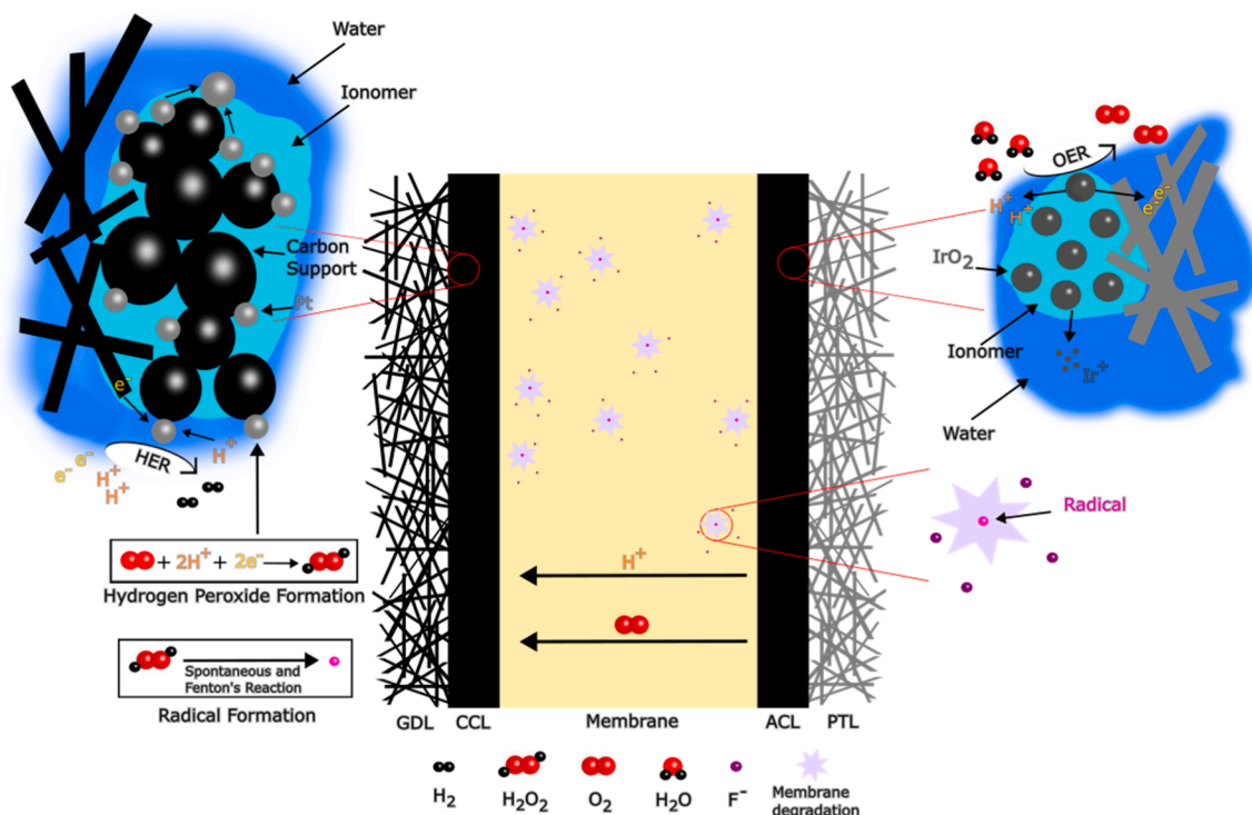
Fig. 2. Main degradation mechanisms considered and evaluated in this study.
