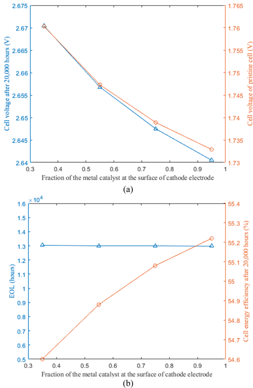
Fig. 27. The impact of varying the fraction of the metal catalyst at the surface of cathode electrode on the (a) cell voltage of pristine cell and degraded cell after 20,000 h (b) EOL and cell energy efficiency after 20,000 h of operation.
