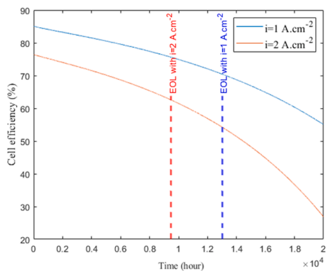
Fig. 16. Variation of cell efficiency when operating the cell at current density of 1 A.cm -2 and 2 A.cm -2 for 20,000 h of operation.
