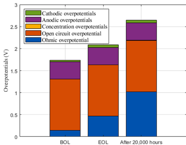
Fig. 14. Contribution of the overpotentials of the cell at the beginning and end of life of the cell.
