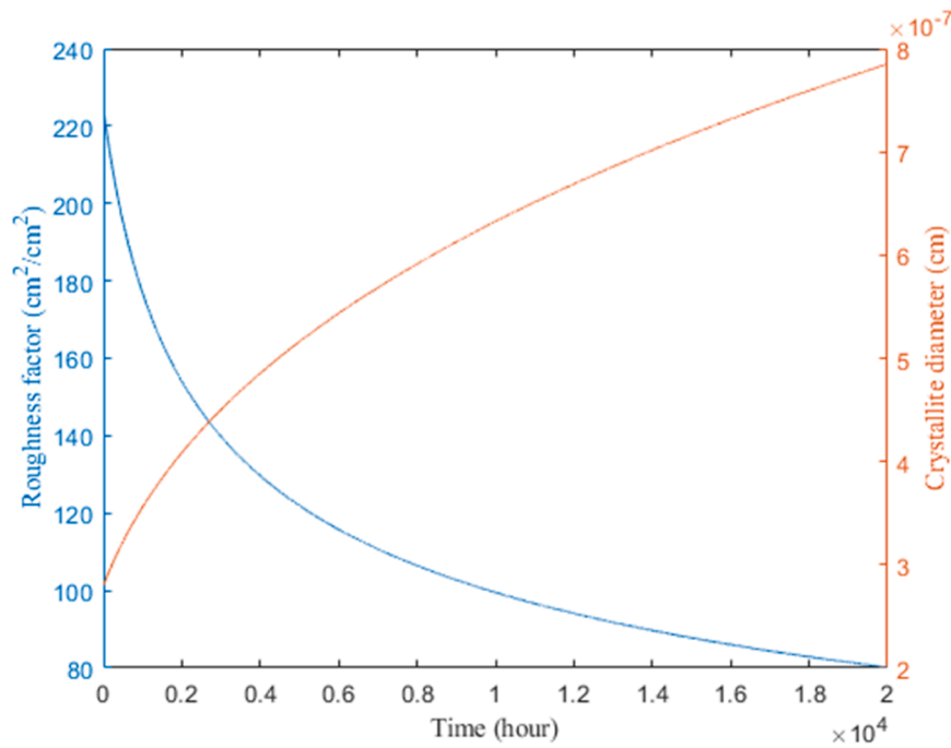
Fig. 10. Variation of roughness factor and crystallite size of the cathode electrode over time.
