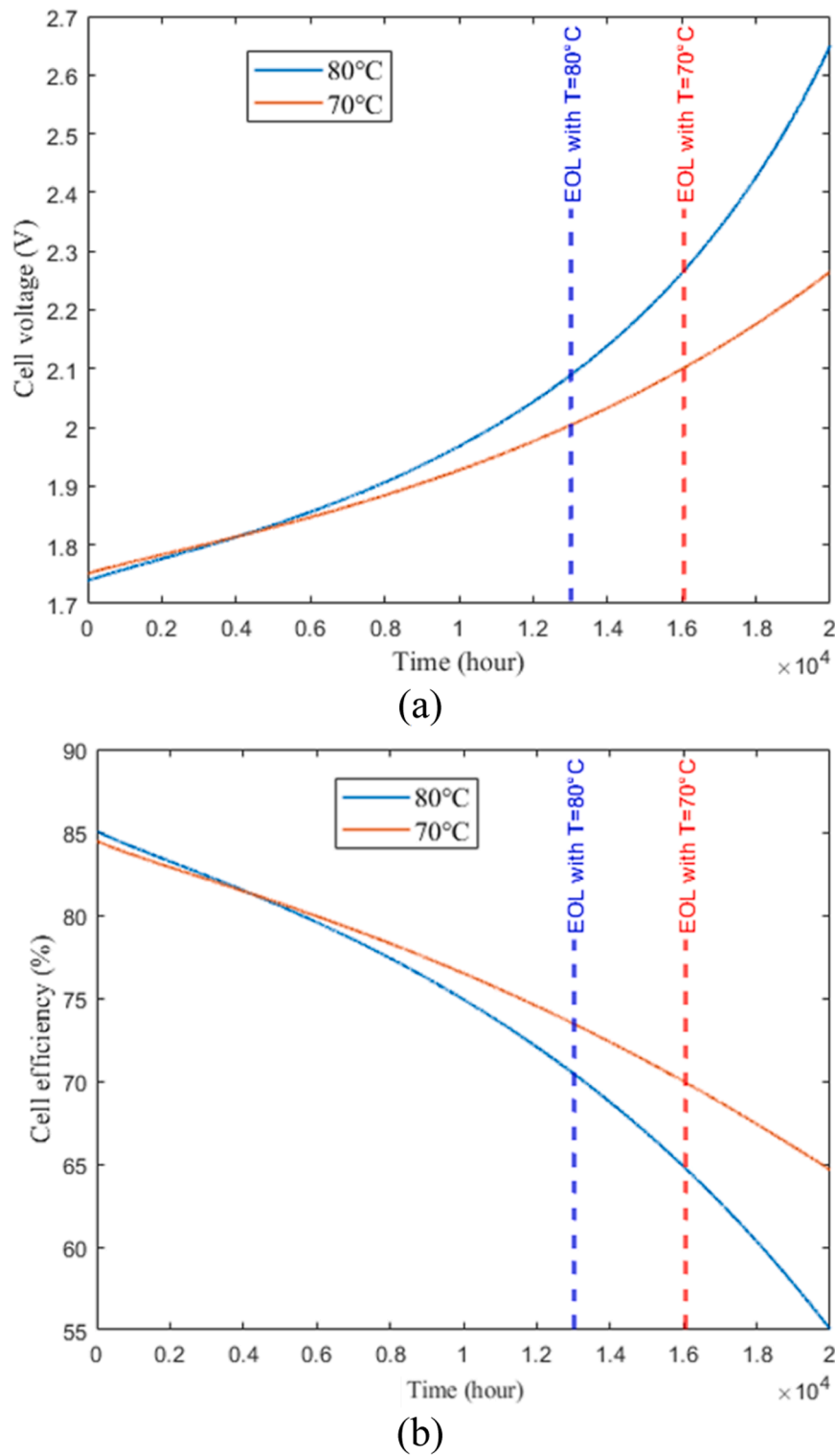
Fig. 24. The impact of operating cell temperature on (a) cell voltage (b) energy efficiency after 20,000 h of operation.
