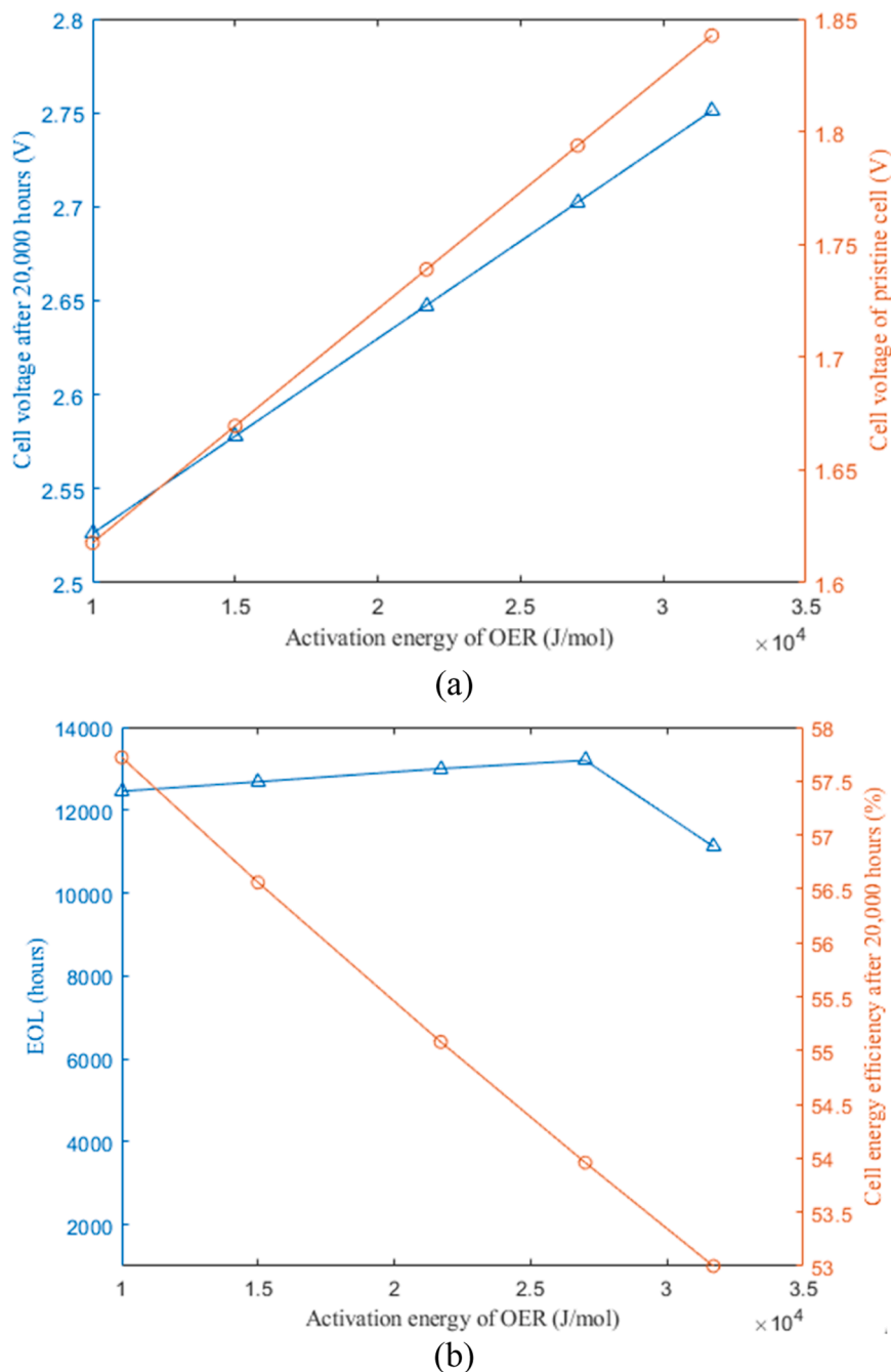
Fig. 26. The impact of varying the activation energy of OER on the (a) cell voltage of pristine cell and degraded cell after 20,000 h (b) EOL and cell energy efficiency after 20,000 h of operation.
