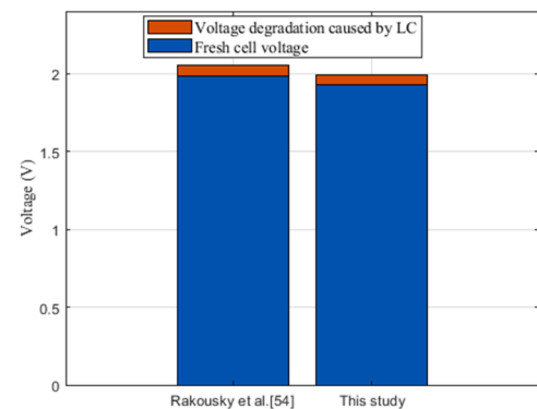
Fig. 19. Validation of the model performance for evaluating the voltage degradation caused by LC.
