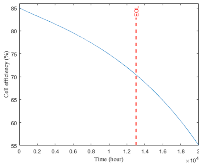
Fig. 13. Variation of cell efficiency when operating under constant load.
