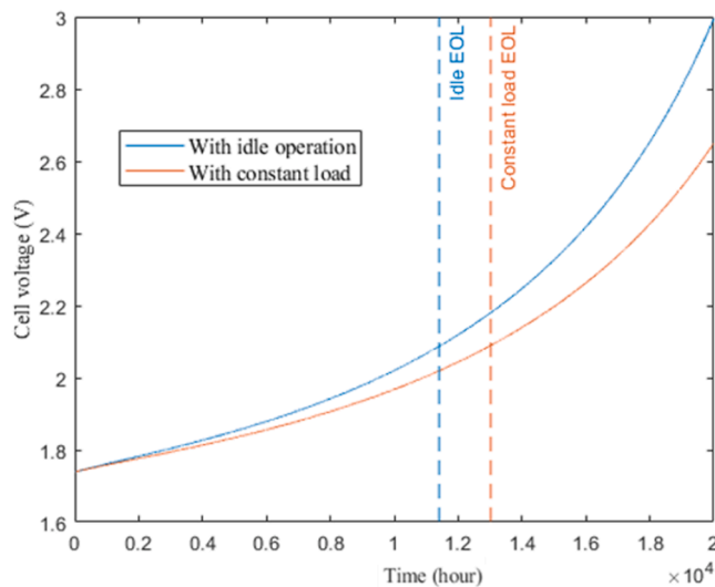
Fig. 22. Comparison of cell voltage degradation and EOL between constant load operation and frequent idle operation.
