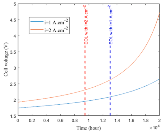
Fig. 15. Variation of cell voltage over time when increasing the current density from 1 A.cm -2 to 2 A.cm -2 .
