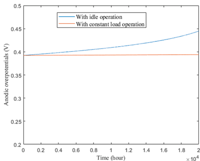
Fig. 20. Comparison of degradation of anodic overpotentials when operating the cell under constant current and frequent idle operation.
