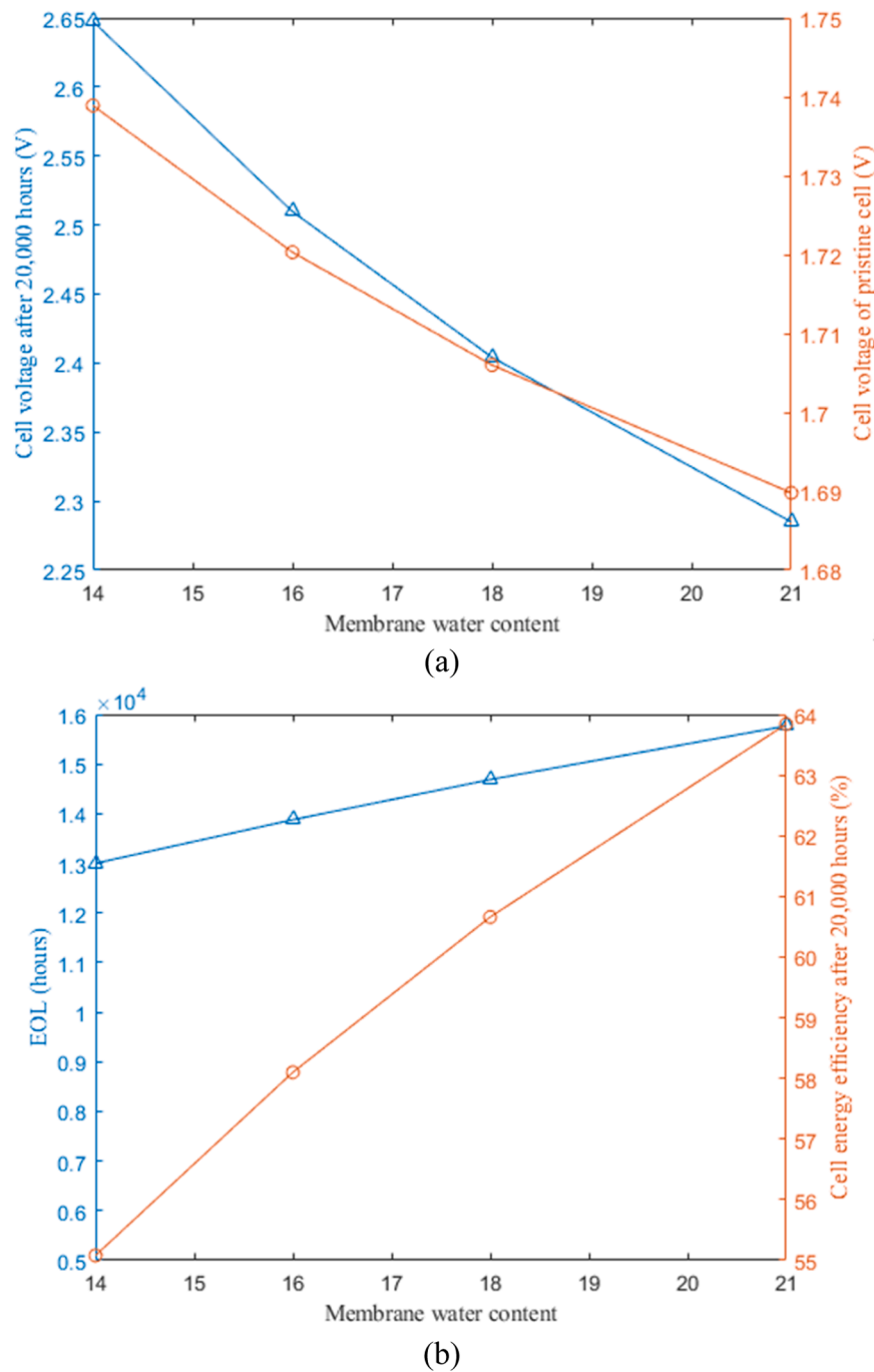
Fig. 28. The impact of varying the membrane water content on the (a) cell voltage of pristine cell and degraded cell after 20,000 h (b) EOL and cell energy efficiency after 20,000 h of operation.
