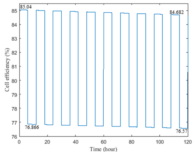
Fig. 18. The impact of LC on the cell efficiency of a PEM electrolysis unit.
