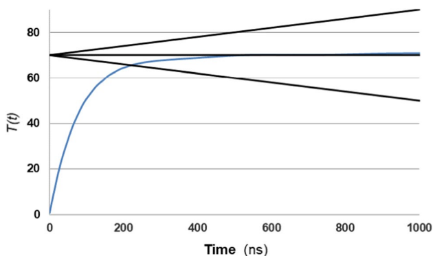
Fig. 6 Integral response of the original divider
