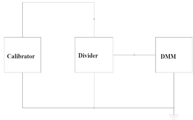
Fig. 9 Scheme of the measurement set-up for the scale factor measurement. The calibrator supplies the divider terminals while the DMM measures the voltage of the low-voltage side of the divider
