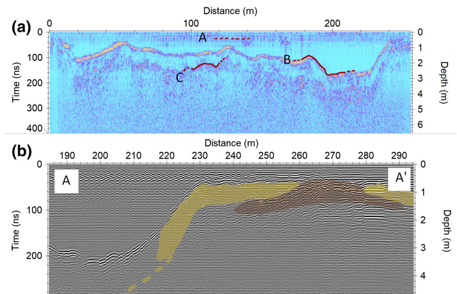
FIGURE 6 (a) Example of a GPR section in which the different reflections are particularly clear. A: Noise due to paddling and boat movement. B: Lake bottom–fine sediment interface. C: Fine sediments–coarse debris interface.
