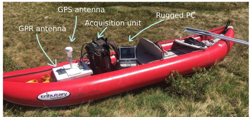
FIGURE B2 The inflatable boat carrying the GPR system. All components are ruggedized and protected from water splashes
