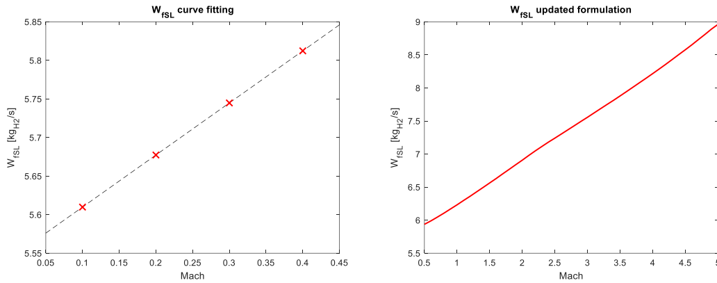
Fig 5. W_{fSL} linear fit and recalculated profile as a function of Mach
