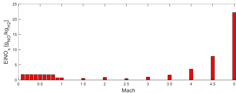
Fig 2. EINO_x from Cantera 0D kinetic-chemical simulations [10]
