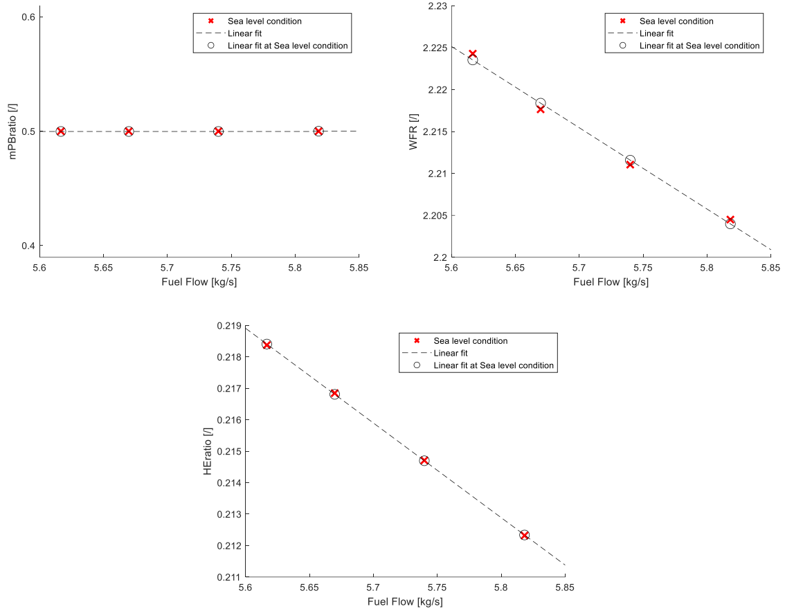
Fig 6. Fits at sea level conditions
