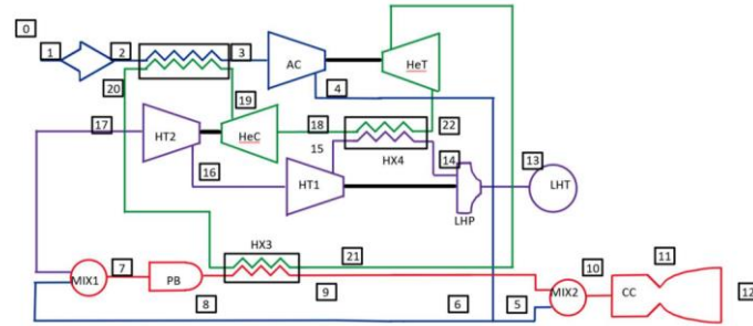
Fig 1. Cycle scheme of the complete model [9]
