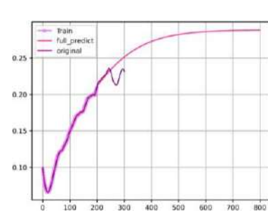
Fig.3: Forecasting of 400 steps
