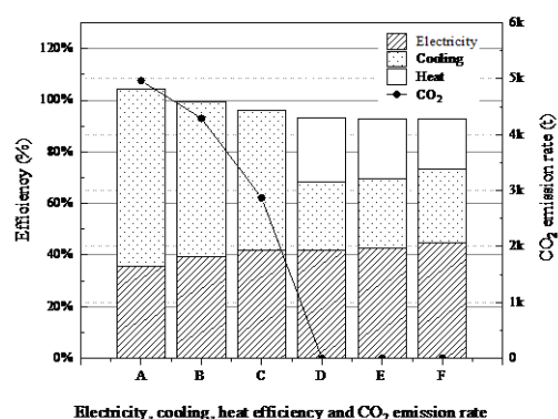
Fig. 2 Results of operational optimization
