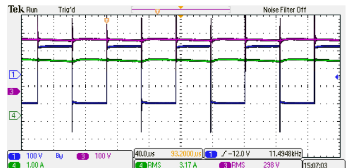
Fig. 14: Sample waveforms for an output of 960W, V_{out} = 300V (Channel 3), I_{out} = 3.2A (Channel 4), output of the bridge (Channel 1)
