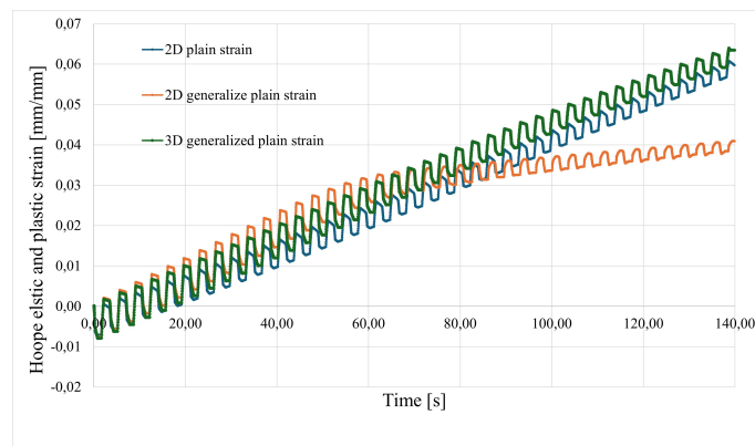
Figure 14: Hoop plastic and elastic strain over time at Point A for different numerical models.
