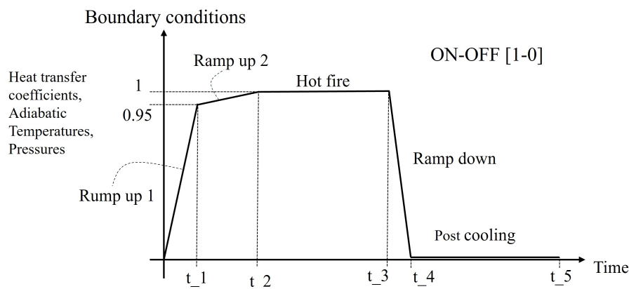
Figure 8: Numerical nominal cycle.
