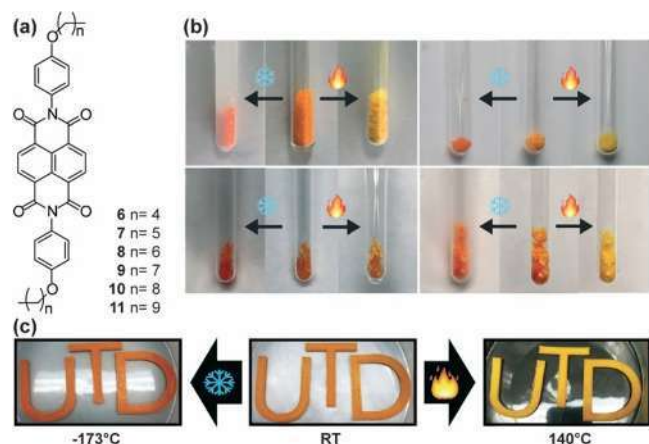
Figure 5. (a) Structure of NDI with various alkyl chains. (b) Thermochromic behavior of 7, 9, 10, and 11 at 100 and -173\text{ }^{\circ}\text{C} . (c) Reversible thermochromic behavior of composite between PLA and crystals of 6. Adapted from ref 110 with permission from The Royal Society of Chemistry.
