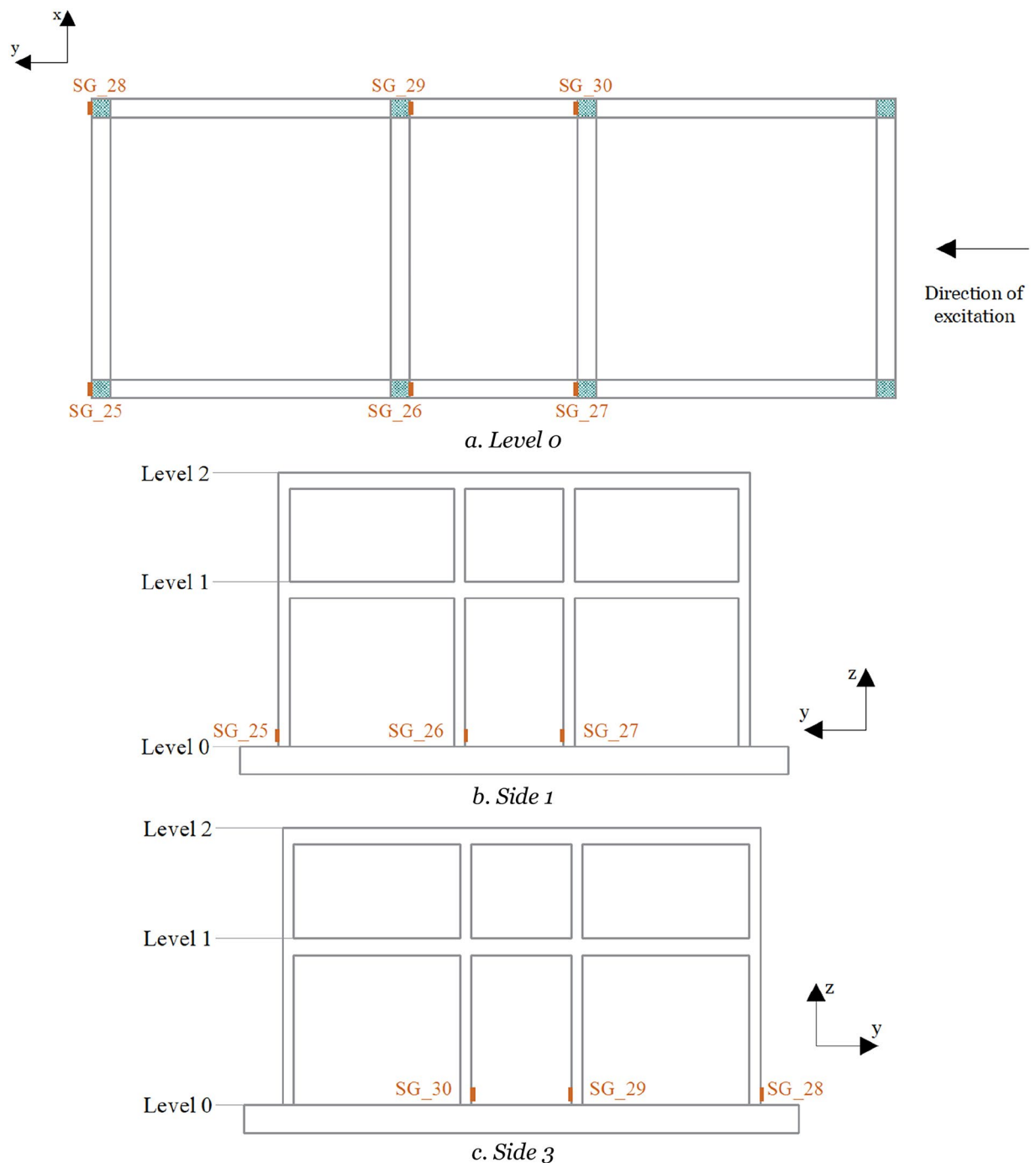
Fig. 11 Strain gauges (SG) on concrete.
