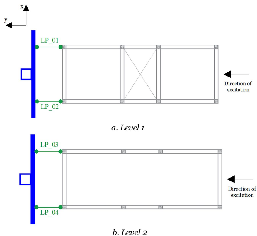
Fig. 8 Linear potentiometers (LPs).
