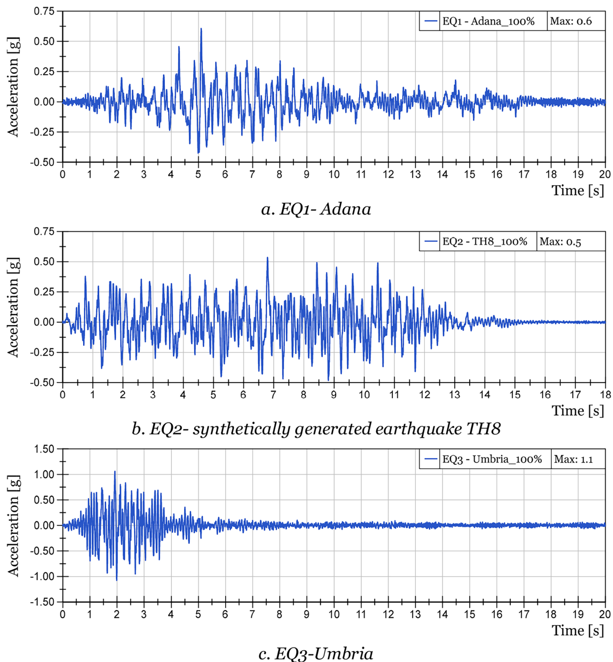
Fig. 12 Time history record of selected ground motions.
