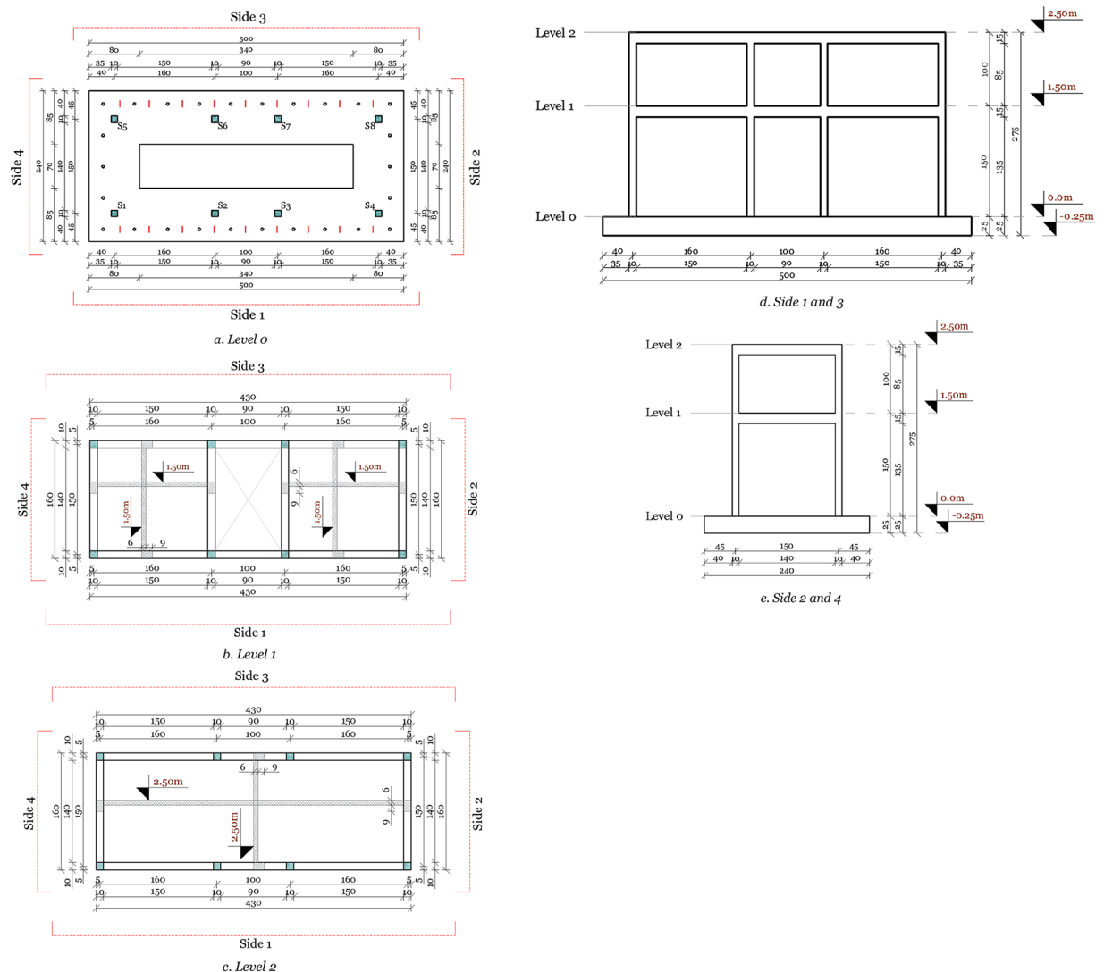
Fig. 1 Technical drawings of the specimens.
