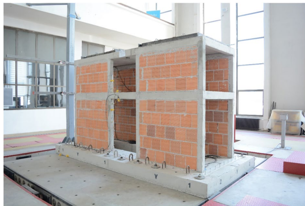
Fig. 2 Unstrengthened RC specimen.
