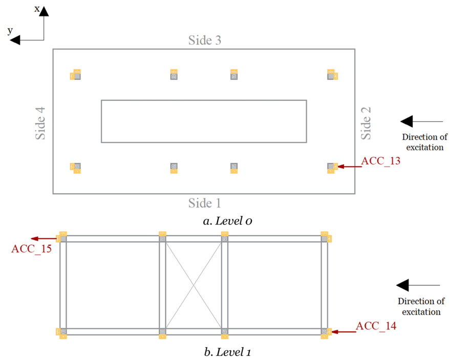
Fig. 7 Accelerometers (ACC) on timber frame.
