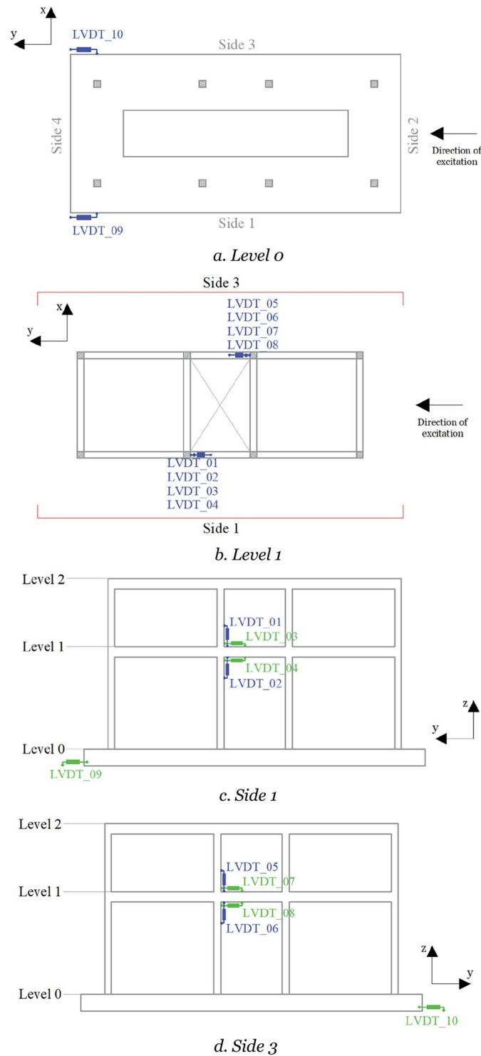
Fig. 9 Linear variable differential transformers (LVDT).
