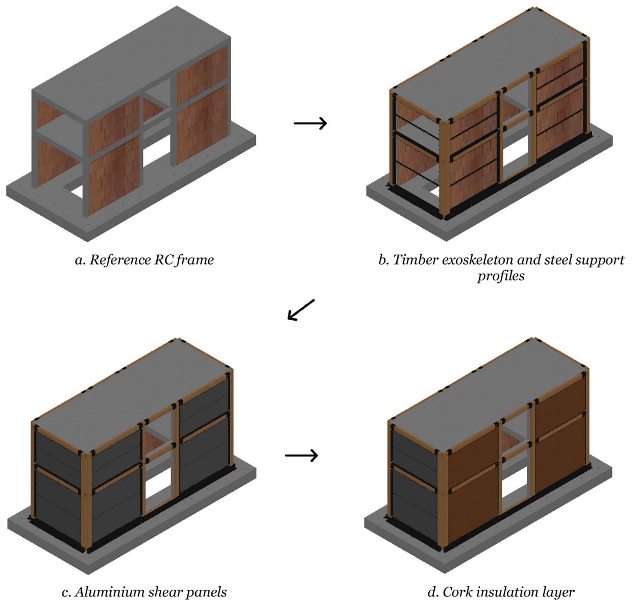
Fig. 3 Exoskeleton installation sequence.
