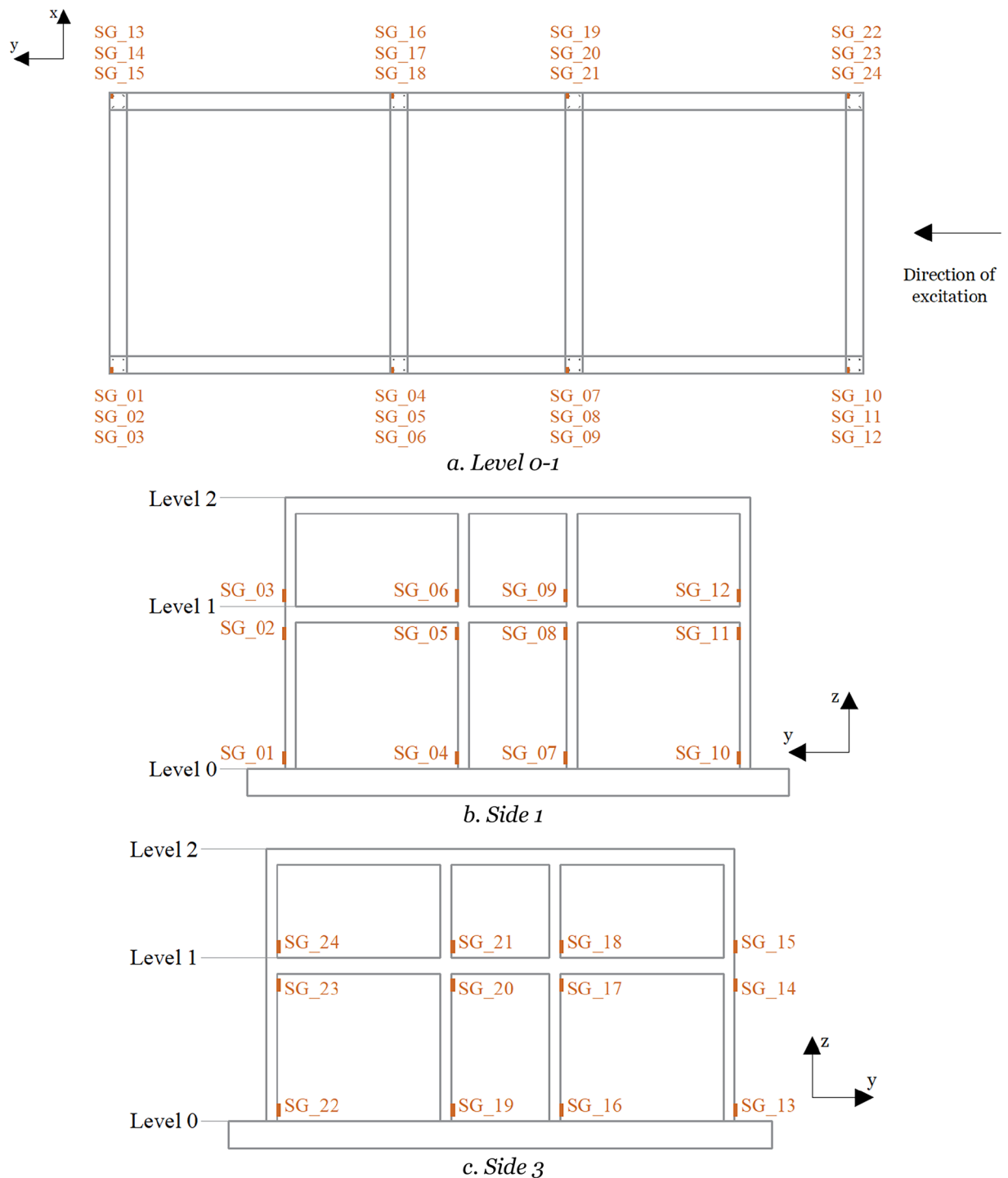
Fig. 10 Strain gauges (SG) on reinforcing bar.
