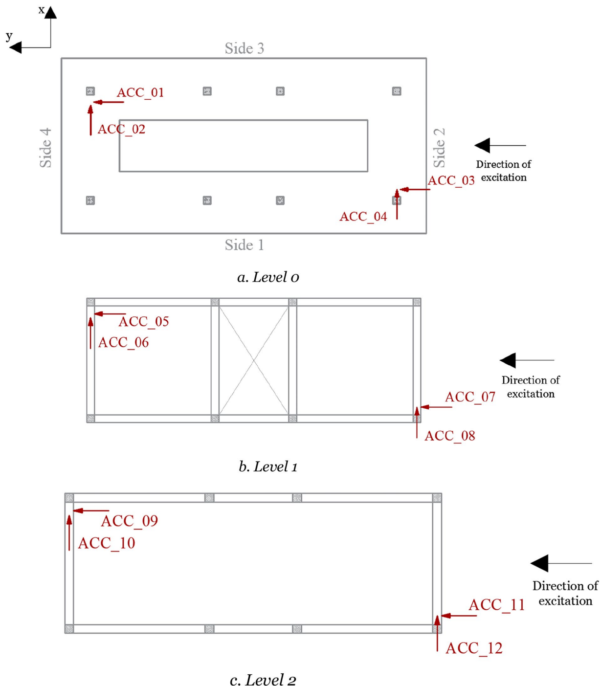
Fig. 6 Accelerometers (ACC) on concrete frame.
