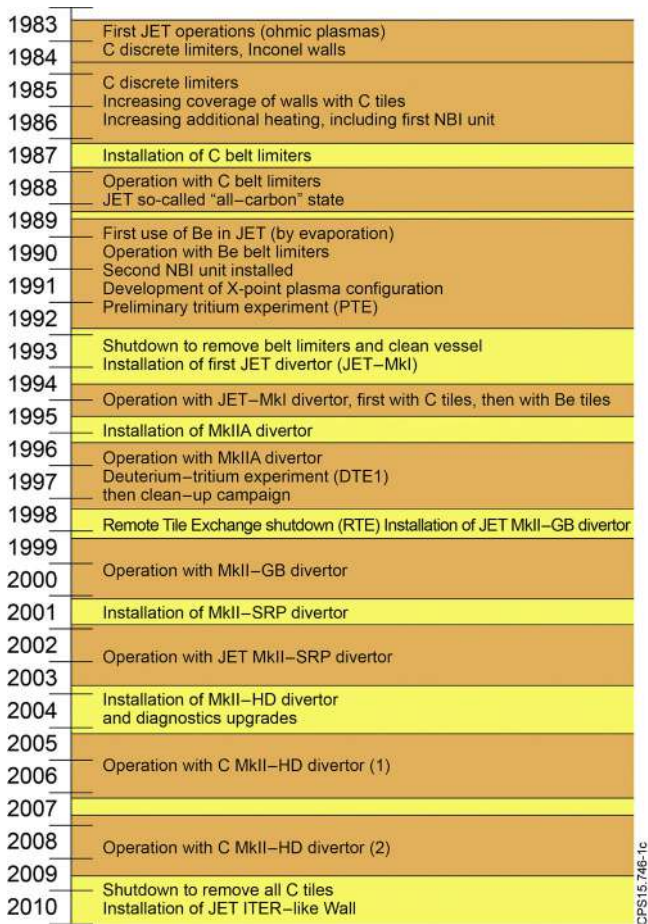
Fig. 1. Timeline for JET operations from the first plasma in 1983 until the removal of the carbon divertor in 2010.
