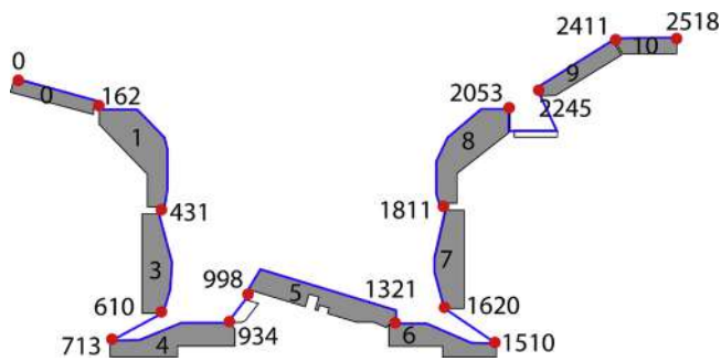
Fig. 13. The cross-section of the JET HD divertor showing the agreed s co-ordinate system for specifying the poloidal locations of the surfaces of the divertor tiles. When applied retrospectively to the MkII-SRP divertor, the SRP (which fits directly between Tiles 4 and 6) has co-ordinates for its top surface from 980 to 1260 mm.
