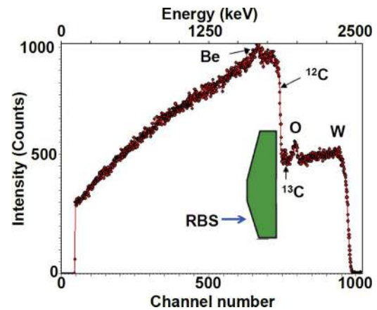
Fig. 27. An RBS spectrum from the W stripe about one-third the way up the Tile 7 surface as shown in the sketch, after exposure in JET 2001–4. Edges labelled W and ^{12}\text{C} are the high energy edge of the feature characteristic of that element. Small amounts of Be, ^{13}\text{C} and O are also present at the surface.
