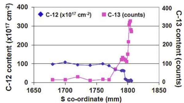
Fig. 57. Plot of ^{13}\text{C} and ^{12}\text{C} measured by NRA across Tile 2ONG7A, showing that the deposit at the top edge is almost exclusively ^{13}\text{C} and not ^{12}\text{C} .
