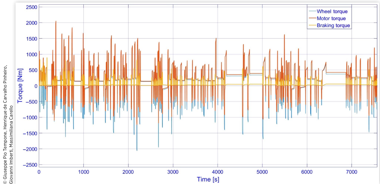
FIGURE 15 Total torque for four motors and four brakes—Test 5.
