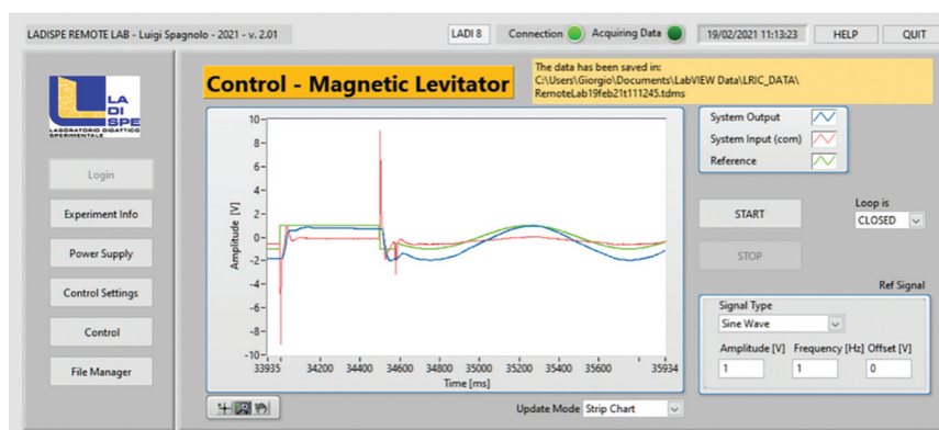
Figure 3. REAL remote user interface.
