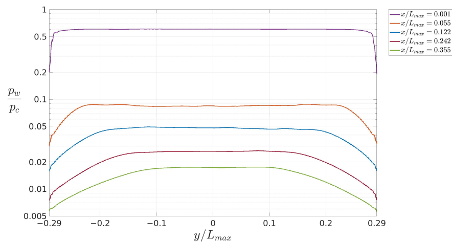
Figure 12. Spanwise wall pressure distributions p_w/p_c at different streamwise locations for \text{NPR} = 200 .
