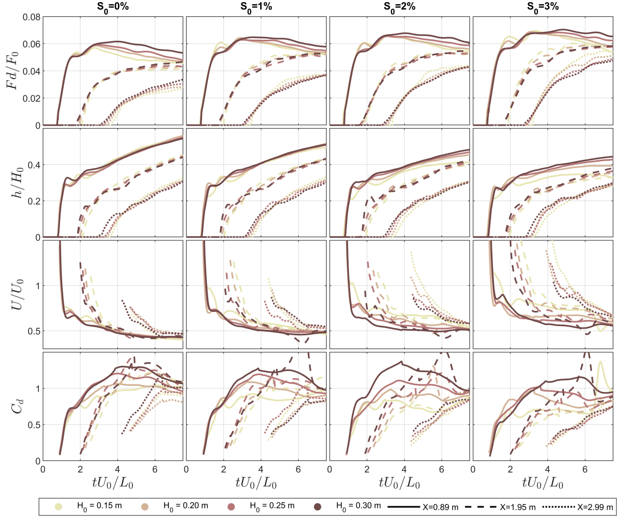
FIG. 4. Variations of the normalized drag, water level, velocity, and C_d as a function of time at the three load cell locations for all H_o and S_o conditions (columns). Here, F_o is the normalizing force computed using C_d = 1 , U_o^2 = gH_o , and \rho = 1000 \text{ kg m}^{-3} .
