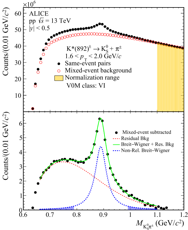
Fig. 1. The K_S^0\pi^\pm invariant mass distribution at |y| < 0.5 in pp collisions at \sqrt{s} = 13 TeV for the 1.6 < p_T < 2.0 GeV/c interval in the VI VOM multiplicity class (black full circles), before (upper panel) and after (lower panel) the uncorrelated background subtraction. Statistical uncertainties are shown with error bars. In the upper panel the red open circles describe the background shape evaluated via the event-mixing technique, while the yellow-filled area represents the normalization region (1.1–1.2 GeV/c 2 ) between the mixed-event background and the same-event pair invariant mass distribution. In the lower panel the solid green curve is the result of the fit with Eq. 1, while the dashed red and blue line describe, respectively, the residual background given by Eq. 2 and the non-relativistic Breit–Wigner function. The blue regions represent the tails of the non-relativistic Breit–Wigner fit outside the integration region.
