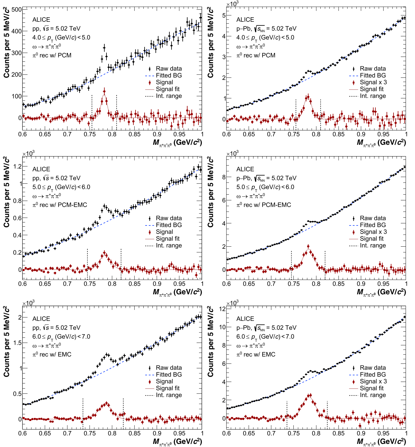
FIG. 1. Invariant mass distributions of \pi^+\pi^-\pi^0 triplets in the indicated p_T ranges for \pi^0 's reconstructed with PCM (top), PCM-EMCal (middle), and EMCal (bottom) in pp (left) and p -Pb (right) collisions. Subtraction of the third-order polynomial background description (blue) from the \pi^+\pi^-\pi^0 candidates (black) results in the signal of \omega candidates (red). In p -Pb collisions, this signal is scaled by a factor of three for better visibility. The vertical dashed lines denote the invariant mass region where the raw yield was obtained through bin counting, as described in Sec. V.
