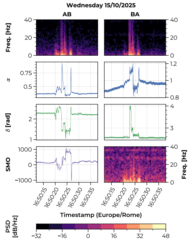
Fig. 12. Event of Wednesday 2025 October 15th, 16:50. Left column: AB direction, Right column: BA direction. 1st row: time spectrogram. 2nd/3rd rows: Polarimeter Jones \alpha and \delta traces. 4th row: SMO device time trace (left) and time spectrogram (right).
