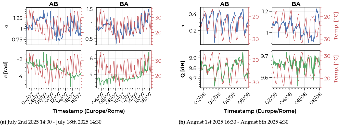
Fig. 11. SOP/Q-Factor vs Temperature taken in (a) July 2025 using setup 2 without SMO card and (b) August 2025 using setup 1 filtered with a 4th order Butterworth filter with 14 mHz bandwidth. Left columns: AB direction, Right columns: BA direction. 1st rows: Polarimeter Jones \alpha trace. 2nd (a) row: Polarimeter Jones \delta trace. 2nd (b) row: Q-factor in dB from transceiver BER. Left y-axes show the recorded temperature (Celsius) of nearby weather station. Time axis is shared and each labeled tick corresponds to the day's midnight.
