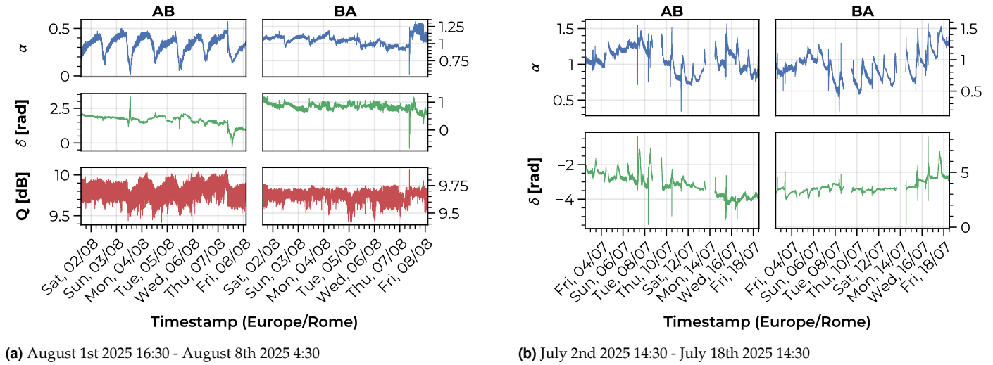
Fig. 9. Experimental measurements taken in (a) August 2025 using setup 1 and (b) July 2025 using setup 2 without SMO card. Left columns: AB direction, Right columns: BA direction. 1st/2nd rows: Polarimeter Jones \alpha and \delta traces. 3rd (a) row: Q-Factor (dB) from transceiver BER. Time axis is shared and each labeled tick corresponds to the day's midnight.
