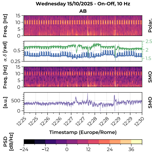
(a) Event of Wednesday 2025 October 15th, 12:25 (AB direction only). 1st: Polarimeter time spectrogram. 2nd: Polarimeter Jones \alpha (blue) and \delta (green) traces. 3rd: SMO device time spectrogram. 4th: SMO device time trace.
