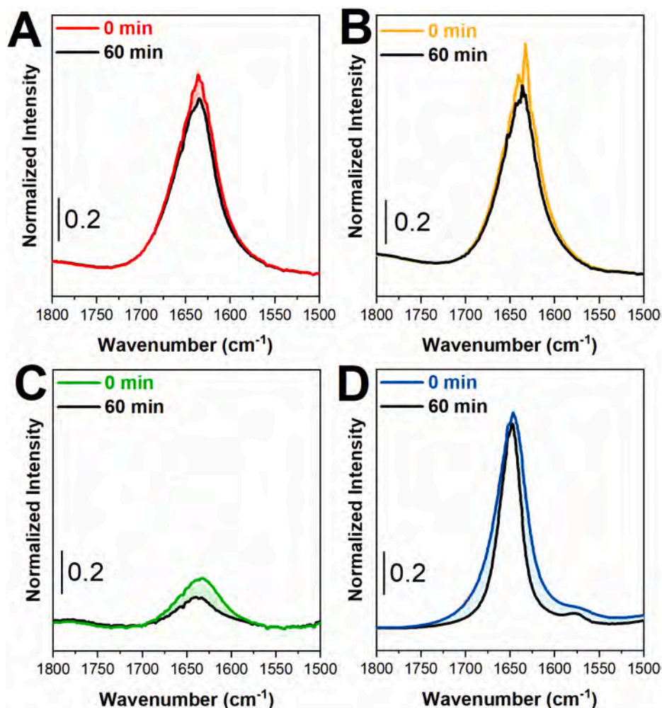
Fig. 12. Time-dependent degassing in situ FTIR spectra of the water interacting region (1800–1500 cm -1 ) acquired on Clino (A), Na/Clino_L (B), Na/Clino_H (C), and 13X (D).
