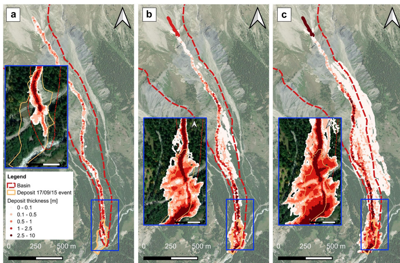
Fig. 11 Comparison between depositional thickness for S1 (a), S2 (b) and S3 (c), using the best-fit rheological parameters ( \mu=0.15 and \xi=500 \text{ m/s}^2 )
