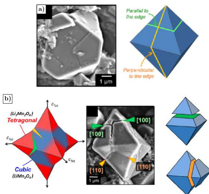
Figure 11. (a) Cubic and (b) tetragonal structure of LMO with the corresponding preferential cracks directions. Reprinted with permission by American Chemical Society from [83], Copyright 2021.
