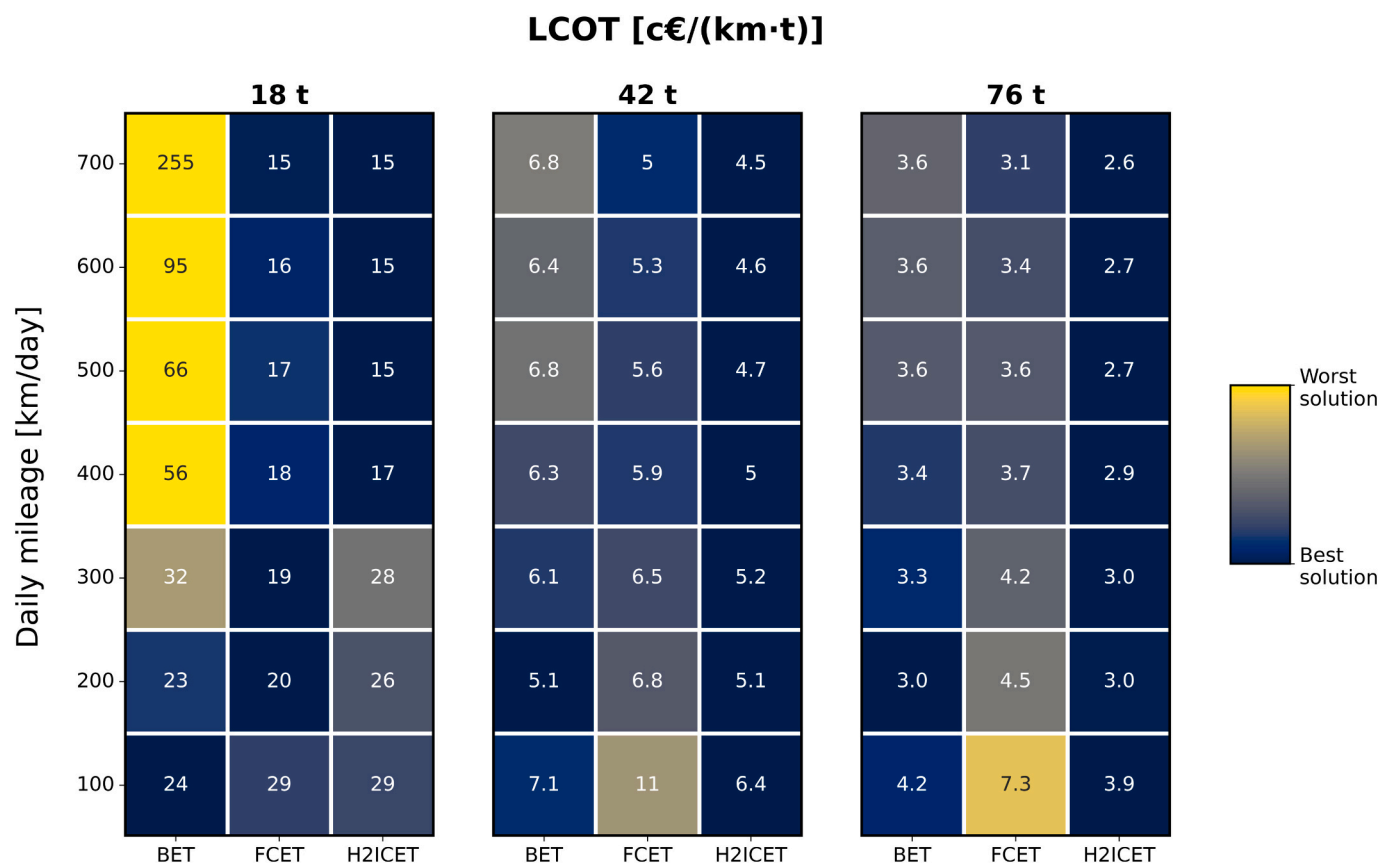
Fig. 6. LCOT (in c€/km·t) for the three powertrain technologies (BET, FCET and H2ICET), for three truck gross weights (18, 42 and 76 t) and variable daily mileages (100 to 700 km/day). The colour of the cells represents the level of cost-competitiveness of the selected combination of weight and daily mileage according to the LCOT indicator, from cost-optimal solutions, in dark blue colour, to the worst cases, in yellow colour. Grid electricity price is assumed equal to 0.10 €/kWh (0.35 €/kWh in fast recharging spots) and hydrogen price equal to 5 €/kg. (For interpretation of the references to colour in this figure legend, the reader is referred to the web version of this article.)
