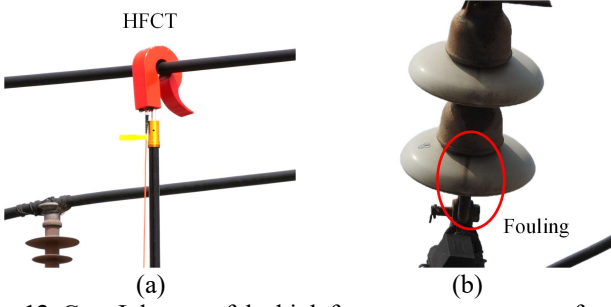
Fig. 13. Case I: layout of the high frequency current transformer on a 10-kV CC line (a) and picture of the PD defect on an insulator caused by fouling (b).
