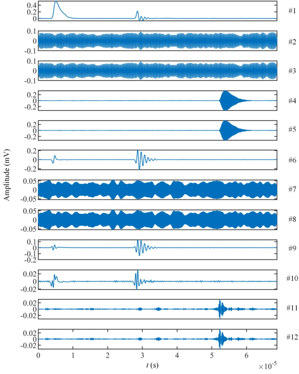
Fig. 6. Signal modes reconstructed from the first twelve components with larger singular values.
