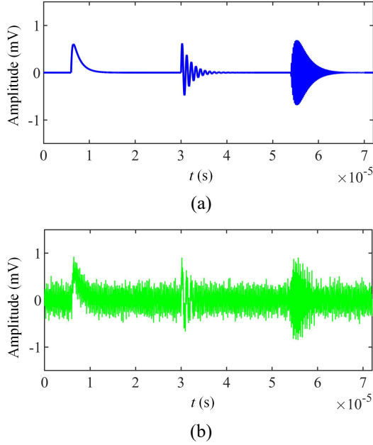
Fig. 1. Synthetic noiseless (a) and noisy (b) PD signal with signal-to-noise ratio of -1.55dB.
