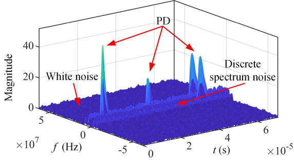
Fig. 3. Magnitude of the spectrogram of the synthetic noisy signal shown in Fig. 1(b) and location of the different signal components.
