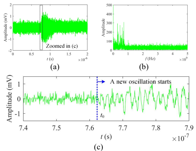
Fig. 17. Case II: time-domain waveform (a) and frequency-domain spectrum (b) of a real noisy PD signal in a 110-kV gas-insulated switchgear, measured by a UHF sensor. The starting of the PD pulse is zoomed in (c).
