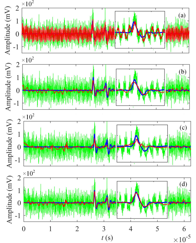
Fig. 15. Case I: de-noising results of real noisy PD signal by (a) H-ASVD (the size of Hankel matrix: 390 \times 7810 ), (b) WT (the mother wavelet: dB8), (c) EMD (the ensemble number: 300), and (d) the proposed STFT-SVD ( M=200 , q=2 ). The green, blue, and red lines denote the noisy, original, and de-noised signal, respectively. The insets zoom in the PD pulses.
