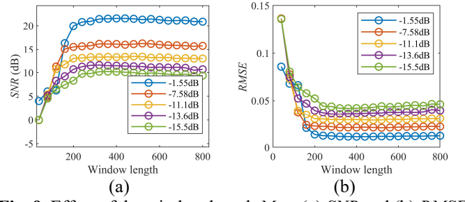
Fig. 9. Effect of the window length M on (a) SNR and (b) RMSE in varying noise levels.
