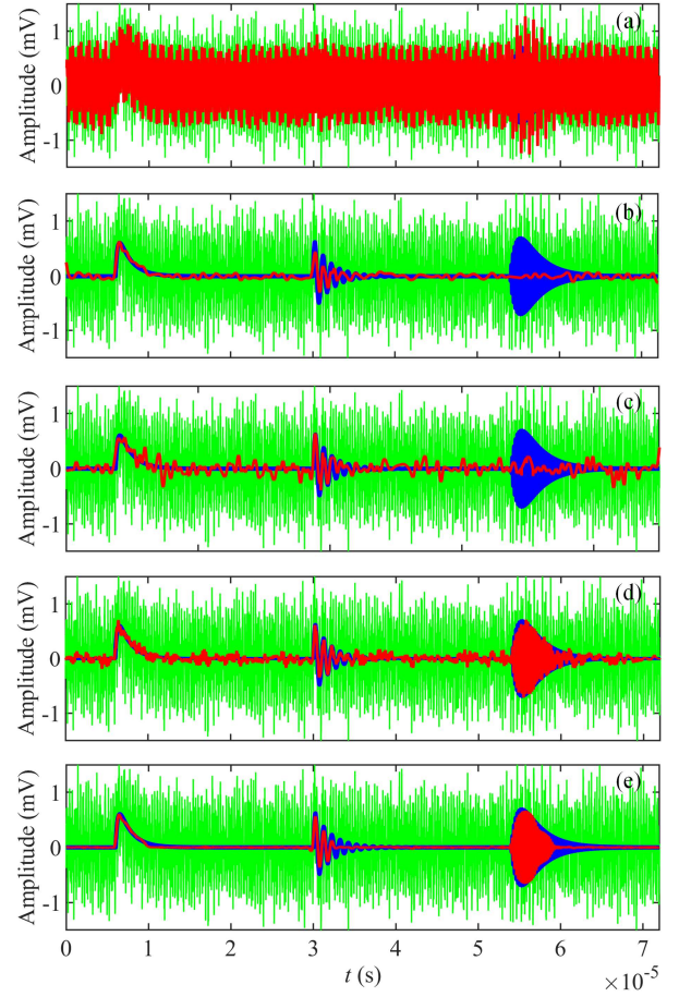
Fig. 12. De-noising results of (a) H-ASVD (the size of Hankel matrix: 450 \times 9000 ), (b) WT (the mother wavelet: dB8), (c) EMD (the ensemble number: 300), (d) the proposed STFT-SVD without the soft masking ( M=200 , q=0 ), and (e) the proposed STFT-SVD with the soft masking ( M=200 , q=2 ). The green, blue, and red lines denote the noisy signal ( SNR=-11.10 dB), the original signal, and the de-noised signal, respectively.
