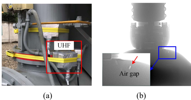
Fig. 16. Case II: layout of a UHF sensor on a 110-kV gas-insulated switchgear (a) and picture of X-ray imaging inspection of the detected internal air gap PD defect of a basin insulator (b).
