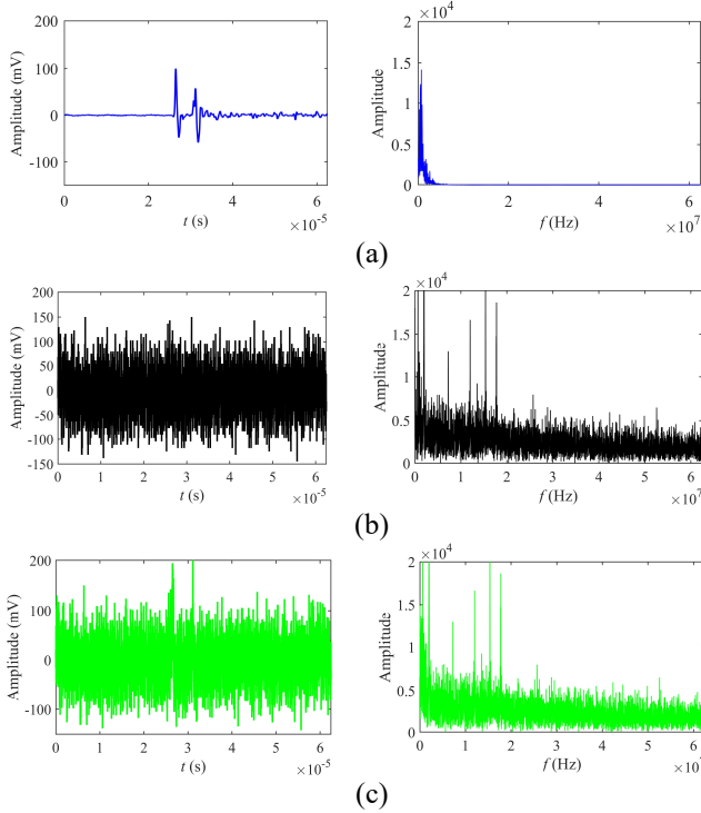
Fig. 14. Case I: time-domain waveforms and frequency-domain spectrums of the HFCT-measured PD signal (a), the HFCT-measured noise (b), and their combination (c).
