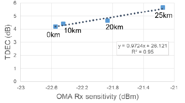
Fig. 5. TDEC against OMA Rx sensitivity for different fiber lengths
