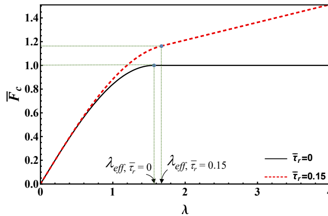
Fig. 3-8. Graphical representation of the maximum load as a function of bond length according to RL for \bar{\tau}_r = 0, 0.15 .
