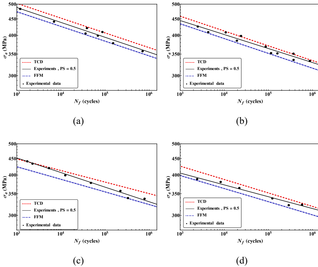
Fig. 5-9. SN Diagrams, featuring both experimental data and forecasts from the TCD and FFM models, for the following configurations: (a) [90/0]_{2s} layup with a notch radius \rho = 2.1 mm, (b) [90/0]_{2s} layup with \rho = 3.25 mm, (c) [0/90]_{2s} layup with \rho = 2.1 mm, and (d) [0/90]_{2s} layup with \rho = 3.25 mm.
