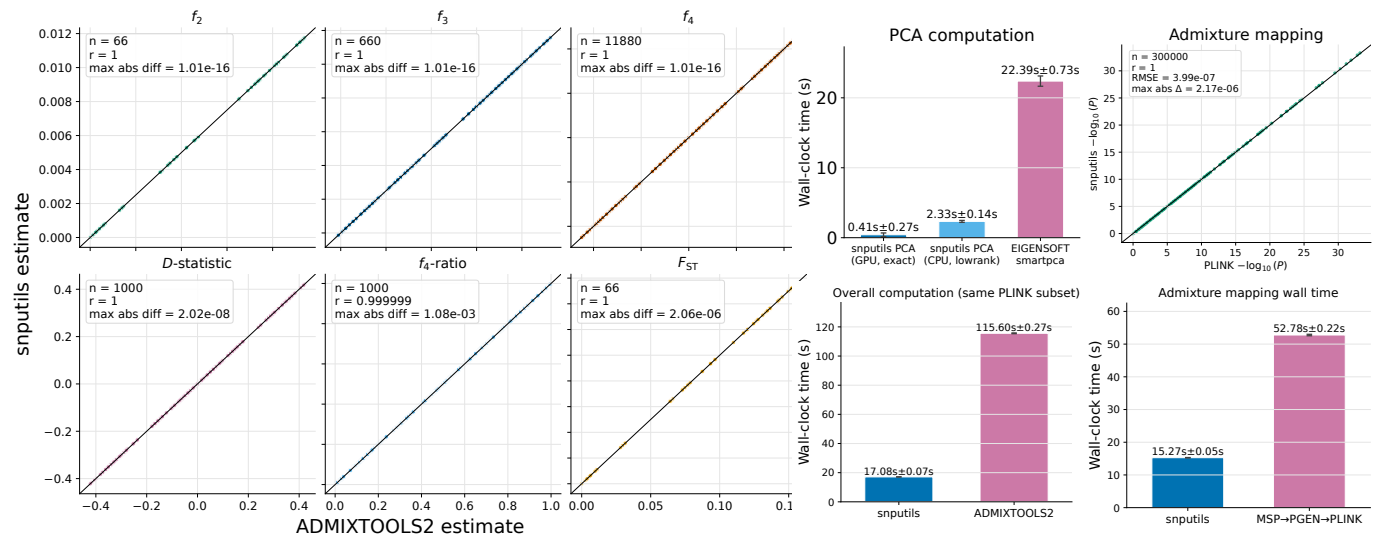
Figure 3 Concordance and runtime benchmarks for allele-frequency statistics, PCA, and admixture mapping. The large left panel shows concordance of allele-frequency-based population statistics computed by snputils and ADMIXTOOLS 2 , including f_2 , f_3 , f_4 , D statistic, f_4 -ratio, and F_{ST} estimates. Points represent matched population configurations, with agreement assessed against the identity line. In the right block, the upper-left panel shows wall-clock runtime for PCA computation using EIGENSOFT smartpca , snputils CPU low-rank PCA, and snputils GPU exact PCA. The lower-left panel shows wall-clock runtime for the complete allele-frequency statistics benchmark using the same PLINK subset on 16 CPUs with 20 GB memory. The upper-right panel shows concordance of admixture mapping association evidence from snputils and PLINK 2 , comparing matched -\log_{10}(P) values across ancestry-window tests. The lower-right panel shows wall-clock runtime for admixture mapping on 16 CPUs with 60 GB memory. Runtime bars show mean \pm standard deviation across five repetitions.
