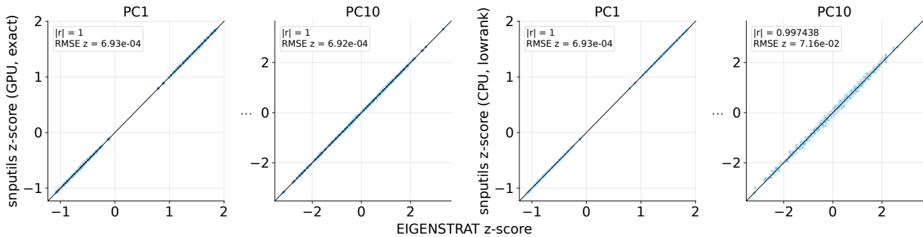
Figure 2 Concordance of standardized PCA sample coordinates from snputils and EIGENSOFT smartpca . The left panels compare snputils GPU exact PCA with EIGENSOFT smartpca , and the right panels compare snputils CPU low-rank PCA with EIGENSOFT smartpca . For each method, component scores were standardized within each principal component and aligned by sign before comparison. Concordance is shown for the first and tenth principal components using matched sample coordinates, with agreement summarized by the absolute Pearson correlation, root mean squared difference in standardized scores, and maximum absolute standardized difference.
