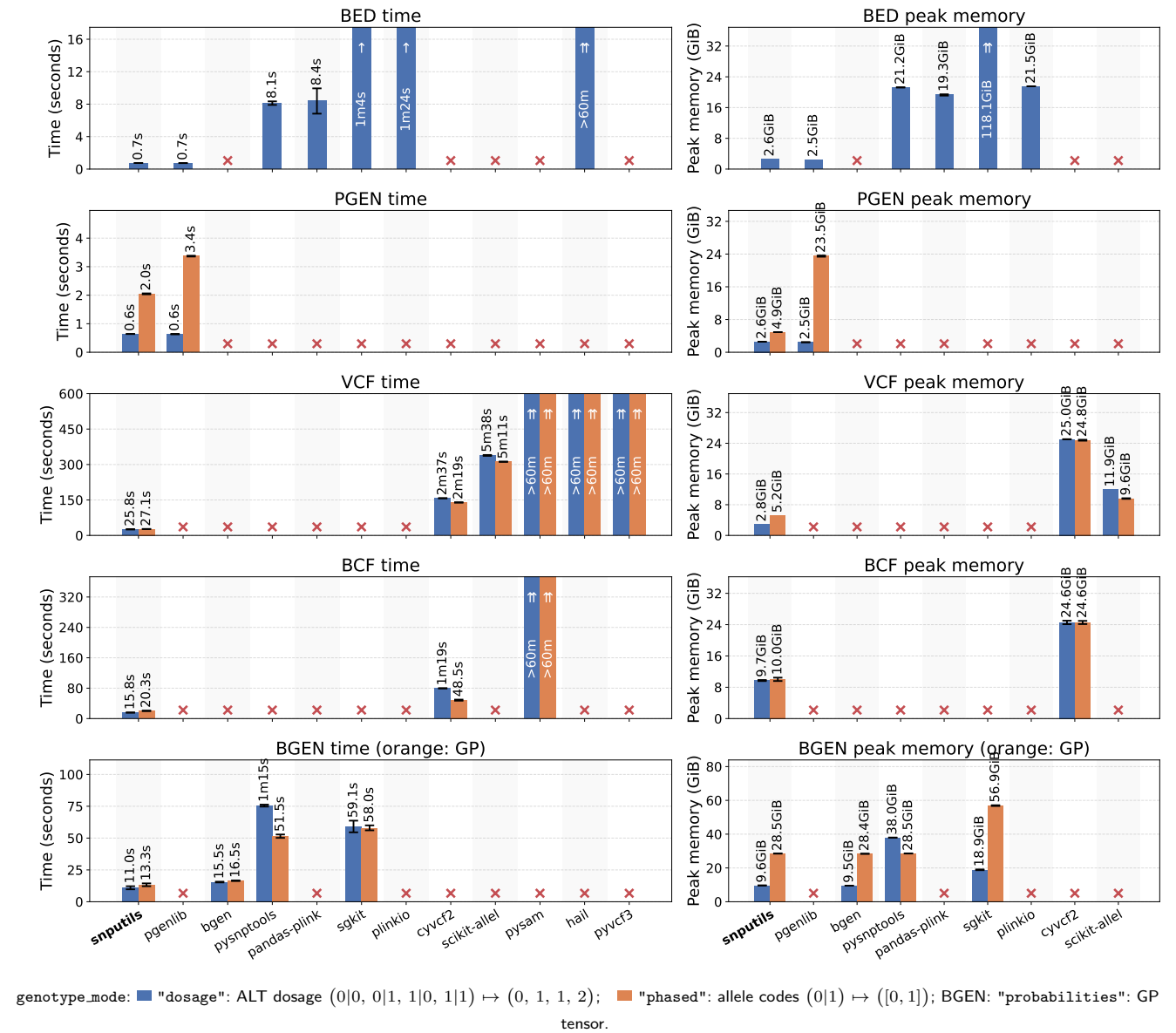
Figure 1 Time and peak memory usage comparison across formats and tools for reading Chromosome 22 SNPs for all samples in the 1000 Genomes Project (The 1000 Genomes Project Consortium, 2015). Blue bars show summed alternate-allele dosages; orange bars show phased allele codes except for BGEN, where they show genotype probability tensors. snputils is fastest and uses the least memory overall, and appears tied with direct pgenlib for summed BED/PGEN dosage timing. Several slow VCF methods are marked as exceeding 60 minutes in the time panel and are omitted from the memory panel because they did not complete a comparable full-read memory profile.
