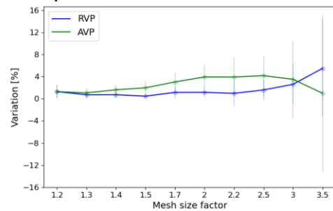
Figure 1: Convergence results of tetra models
