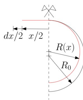
Figure 8. Simplified sketch of the halved brake-ring.
