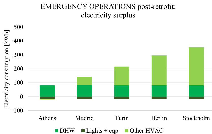
Fig. 9. Breakdown of electricity surplus during the emergency period for the five European locations, post-retrofit.
