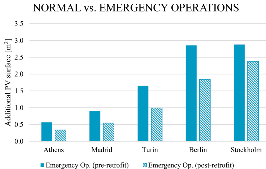
Fig. 10. Additional PV surface needed to meet electricity consumptions in emergency operations w.r.t normal ones, for the five European locations, pre- and post-retrofit interventions.
