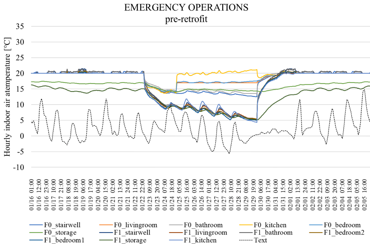
Fig. 5. Hourly external temperature and thermal zones indoor air temperature variation for the SFH located in Turin for emergency operations, pre-retrofit. F0 = ground floor; F1 = first floor.
