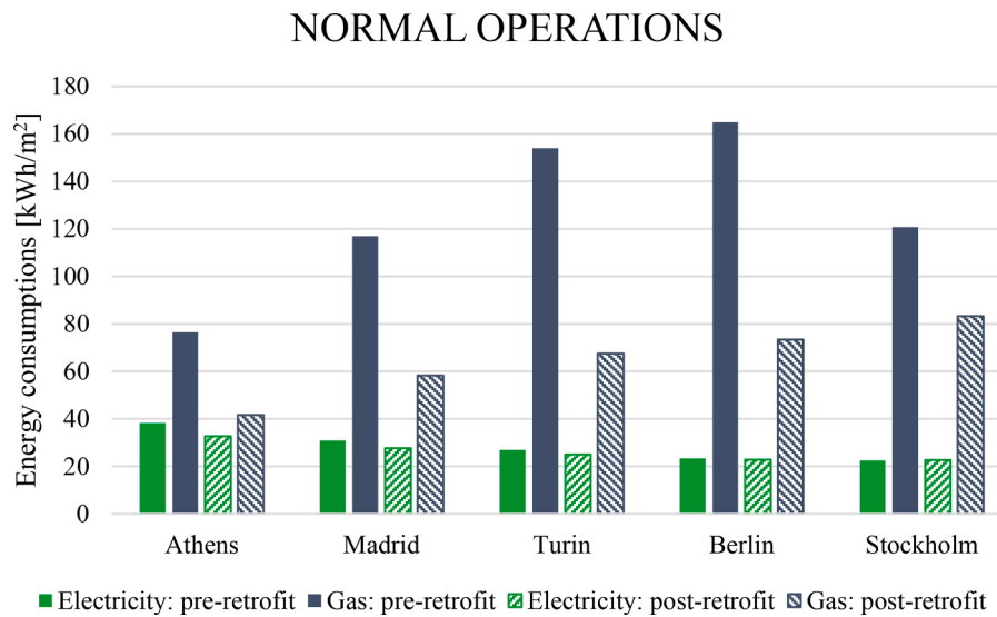
Fig. 6. Simulated electricity and gas consumptions for the five European locations in normal operation, pre- and post-retrofit interventions.
