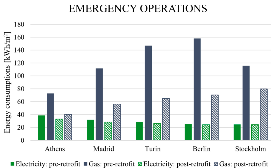
Fig. 7. Simulated electricity and gas consumptions for the five European locations in emergency operation, pre- and post-retrofit interventions.
