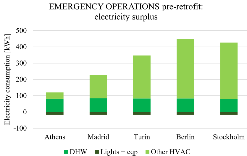
Fig. 8. Breakdown of electricity surplus during the emergency period for the five European locations, pre-retrofit.
